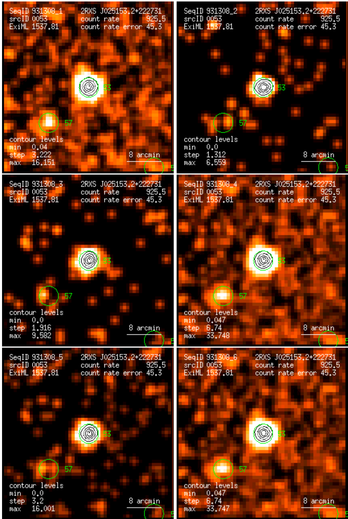
Figure 53: RASS 931308: detection 0053: band rate images, Gaussian filter: (1) PSPC channels 11 – 41, (2) 52 – 90, (3) 91 – 201, (4) 11 – 235, (5) 52 – 201, (6) 11 – 201. Broad band rates in counts/ks. Band rate contour levels in counts/ks/arcmin 2 .
