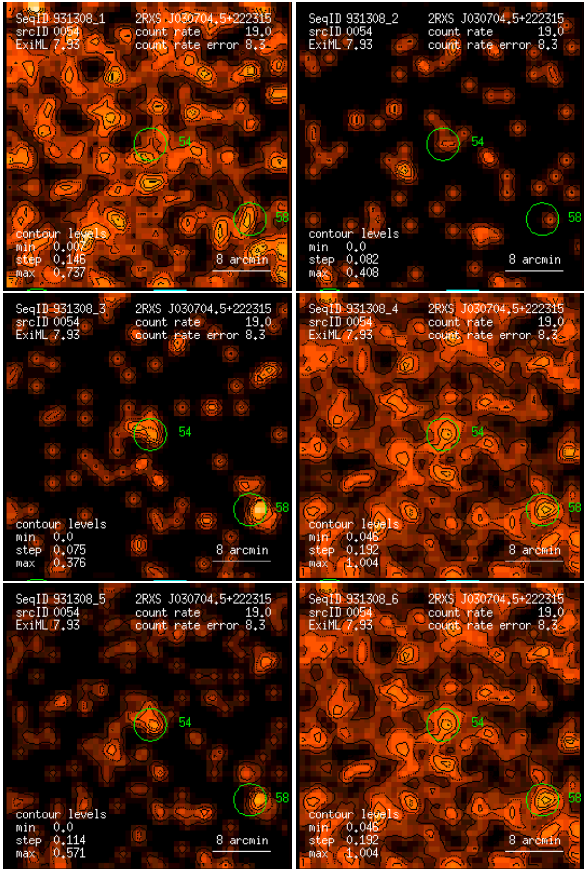
Figure 54: RASS 931308: detection 0054: band rate images, Gaussian filter: (1) PSPC channels 11 – 41, (2) 52 – 90, (3) 91 – 201, (4) 11 – 235, (5) 52 – 201, (6) 11 – 201. Broad band rates in counts/ks. Band rate contour levels in counts/ks/arcmin 2 .
