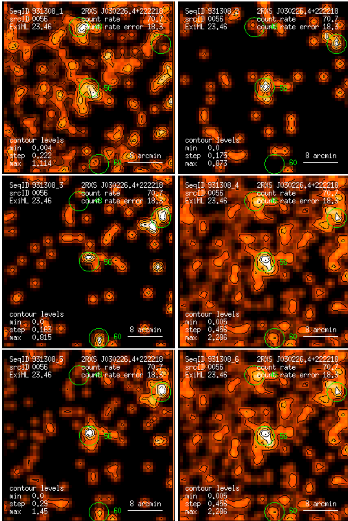
Figure 56: RASS 931308: detection 0056: band rate images, Gaussian filter: (1) PSPC channels 11 – 41, (2) 52 – 90, (3) 91 – 201, (4) 11 – 235, (5) 52 – 201, (6) 11 – 201. Broad band rates in counts/ks. Band rate contour levels in counts/ks/arcmin 2 .
