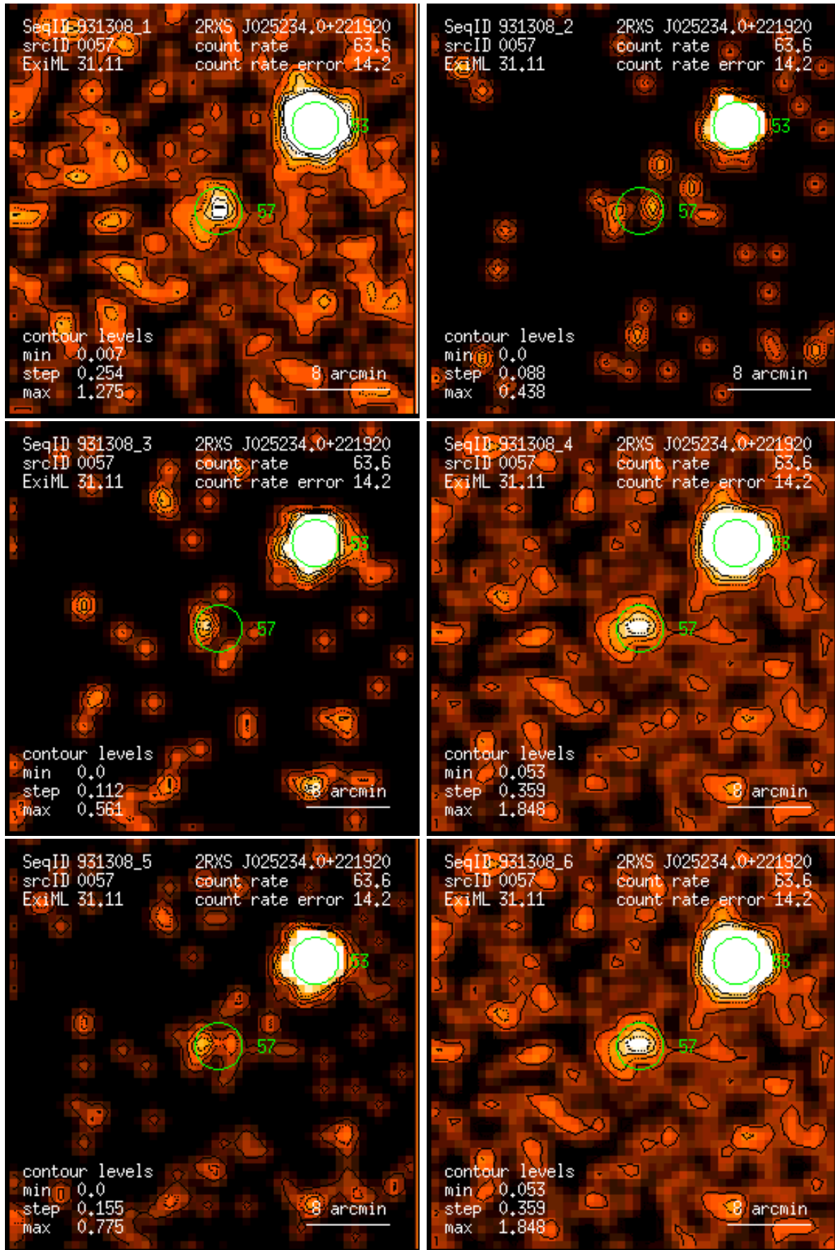
Figure 57: RASS 931308: detection 0057: band rate images, Gaussian filter: (1) PSPC channels 11 – 41, (2) 52 – 90, (3) 91 – 201, (4) 11 – 235, (5) 52 – 201, (6) 11 – 201. Broad band rates in counts/ks. Band rate contour levels in counts/ks/arcmin 2 .
