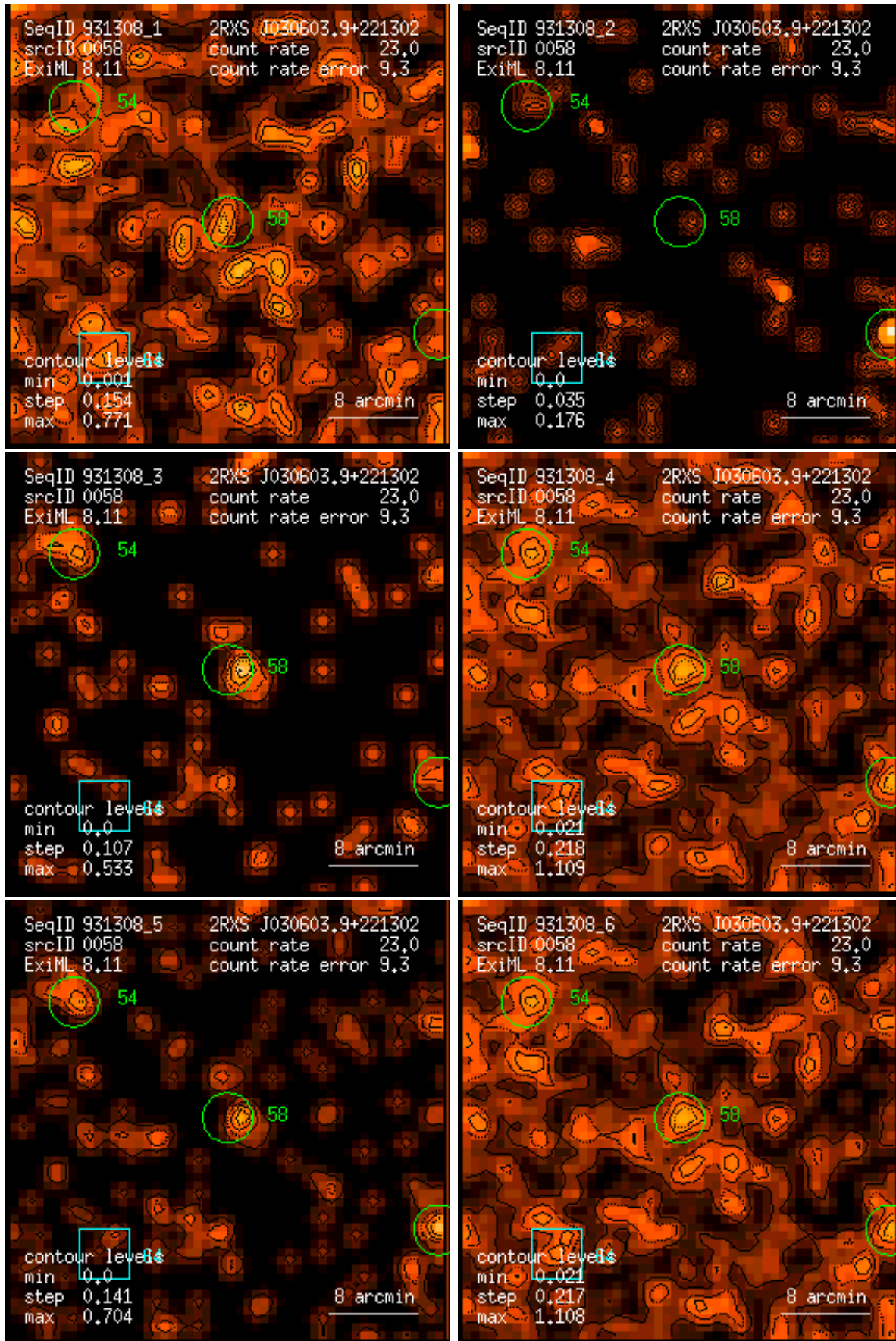
Figure 58: RASS 931308: detection 0058: band rate images, Gaussian filter: (1) PSPC channels 11 – 41, (2) 52 – 90, (3) 91 – 201, (4) 11 – 235, (5) 52 – 201, (6) 11 – 201. Broad band rates in counts/ks. Band rate contour levels in counts/ks/arcmin 2 .
