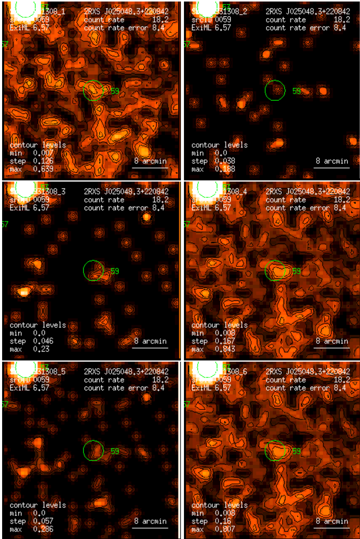
Figure 59: RASS 931308: detection 0059: band rate images, Gaussian filter: (1) PSPC channels 11 – 41, (2) 52 – 90, (3) 91 – 201, (4) 11 – 235, (5) 52 – 201, (6) 11 – 201. Broad band rates in counts/ks. Band rate contour levels in counts/ks/arcmin 2 .
