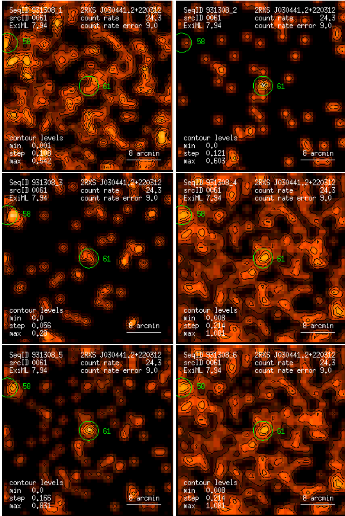
Figure 61: RASS 931308: detection 0061: band rate images, Gaussian filter: (1) PSPC channels 11 – 41, (2) 52 – 90, (3) 91 – 201, (4) 11 – 235, (5) 52 – 201, (6) 11 – 201. Broad band rates in counts/ks. Band rate contour levels in counts/ks/arcmin 2 .
