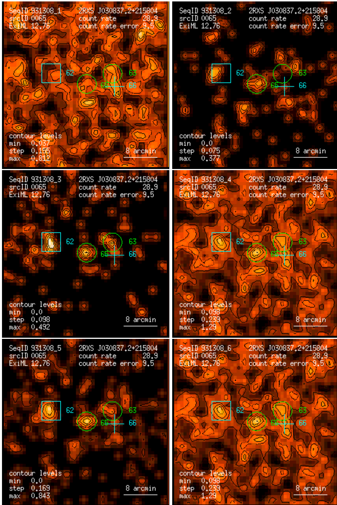
Figure 65: RASS 931308: detection 0065: band rate images, Gaussian filter: (1) PSPC channels 11 – 41, (2) 52 – 90, (3) 91 – 201, (4) 11 – 235, (5) 52 – 201, (6) 11 – 201. Broad band rates in counts/ks. Band rate contour levels in counts/ks/arcmin 2 .
