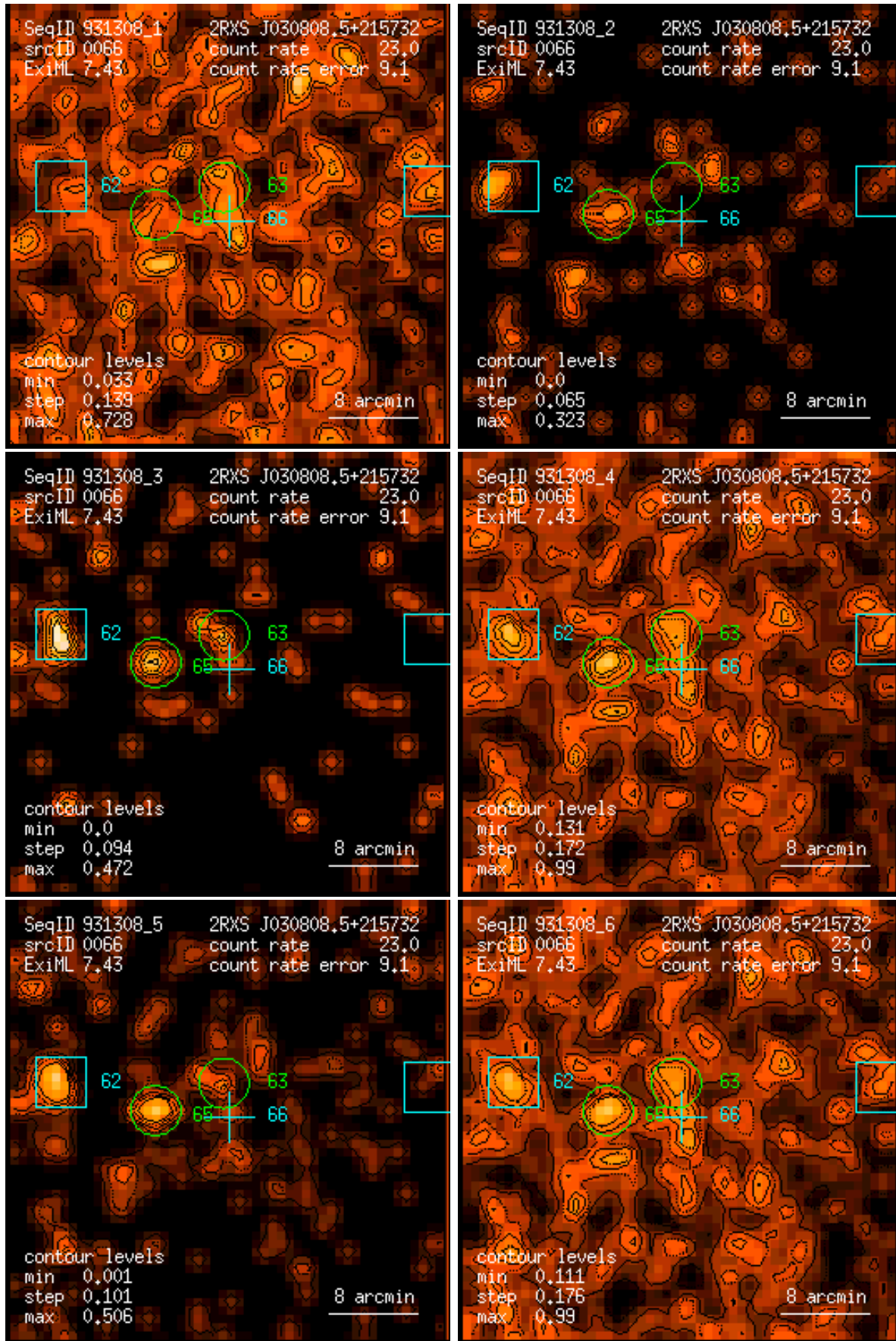
Figure 66: RASS 931308: detection 0066: band rate images, Gaussian filter: (1) PSPC channels 11 – 41, (2) 52 – 90, (3) 91 – 201, (4) 11 – 235, (5) 52 – 201, (6) 11 – 201. Broad band rates in counts/ks. Band rate contour levels in counts/ks/arcmin 2 .
