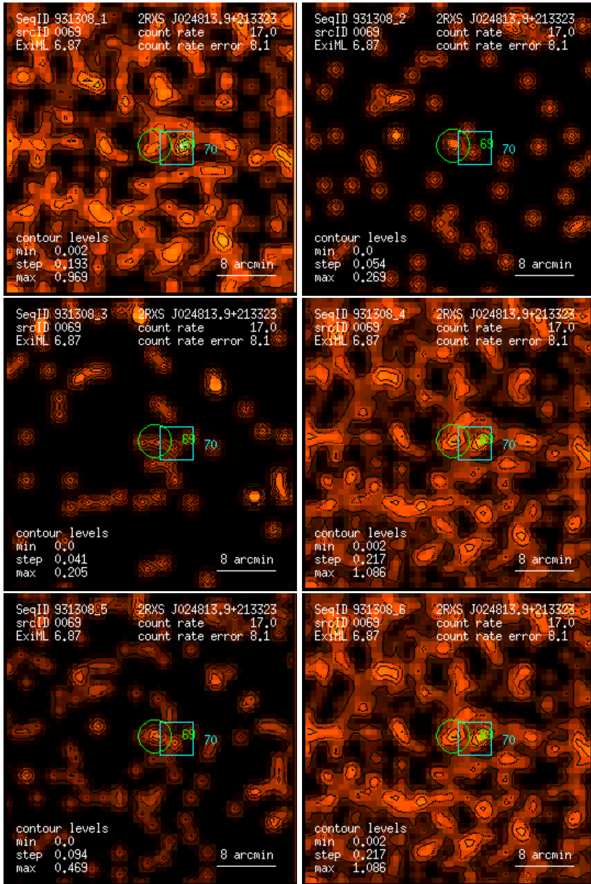
Figure 69: RASS 931308: detection 0069: band rate images, Gaussian filter: (1) PSPC channels 11 – 41, (2) 52 – 90, (3) 91 – 201, (4) 11 – 235, (5) 52 – 201, (6) 11 – 201. Broad band rates in counts/ks. Band rate contour levels in counts/ks/arcmin 2 .
