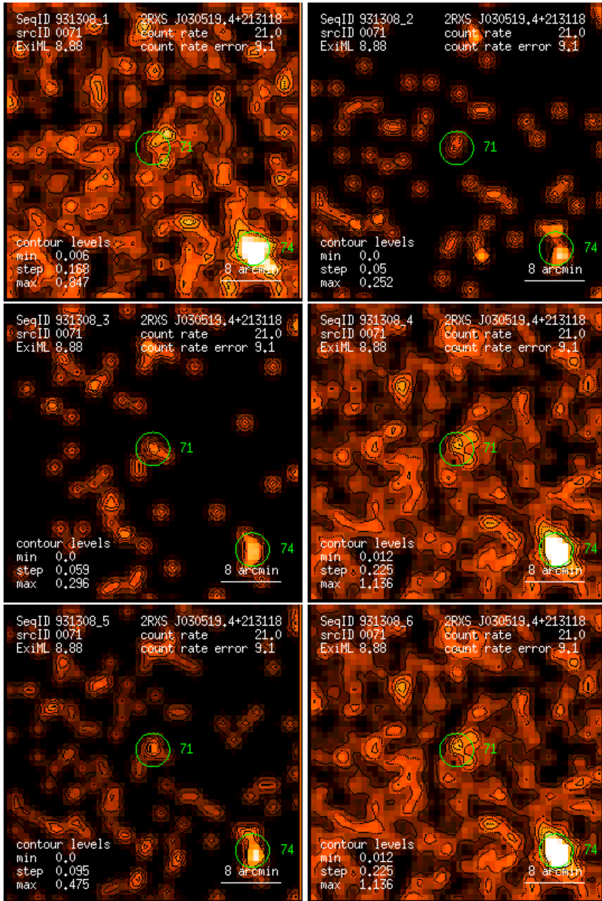
Figure 71: RASS 931308: detection 0071: band rate images, Gaussian filter: (1) PSPC channels 11 – 41, (2) 52 – 90, (3) 91 – 201, (4) 11 – 235, (5) 52 – 201, (6) 11 – 201. Broad band rates in counts/ks. Band rate contour levels in counts/ks/arcmin 2 .
