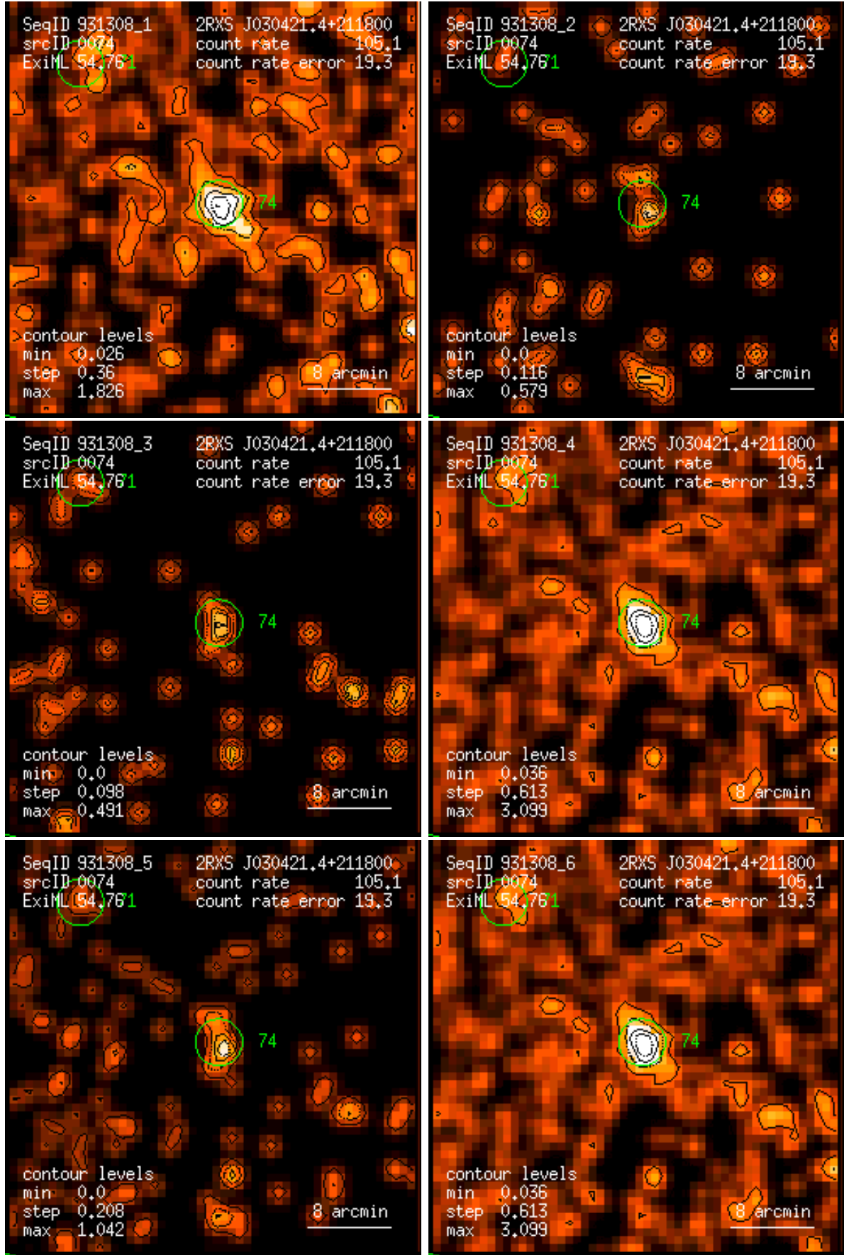
Figure 74: RASS 931308: detection 0074: band rate images, Gaussian filter: (1) PSPC channels 11 – 41, (2) 52 – 90, (3) 91 – 201, (4) 11 – 235, (5) 52 – 201, (6) 11 – 201. Broad band rates in counts/ks. Band rate contour levels in counts/ks/arcmin 2 .
