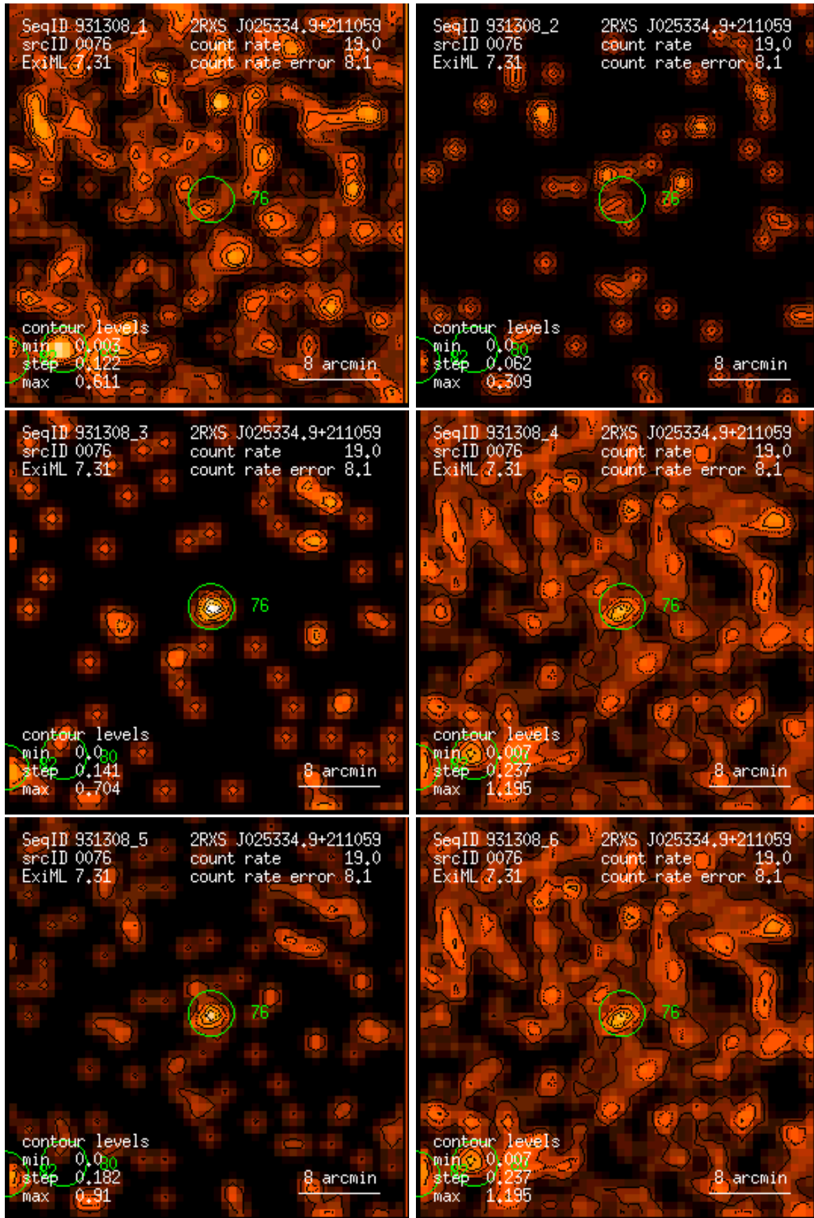
Figure 76: RASS 931308: detection 0076: band rate images, Gaussian filter: (1) PSPC channels 11 – 41, (2) 52 – 90, (3) 91 – 201, (4) 11 – 235, (5) 52 – 201, (6) 11 – 201. Broad band rates in counts/ks. Band rate contour levels in counts/ks/arcmin 2 .
