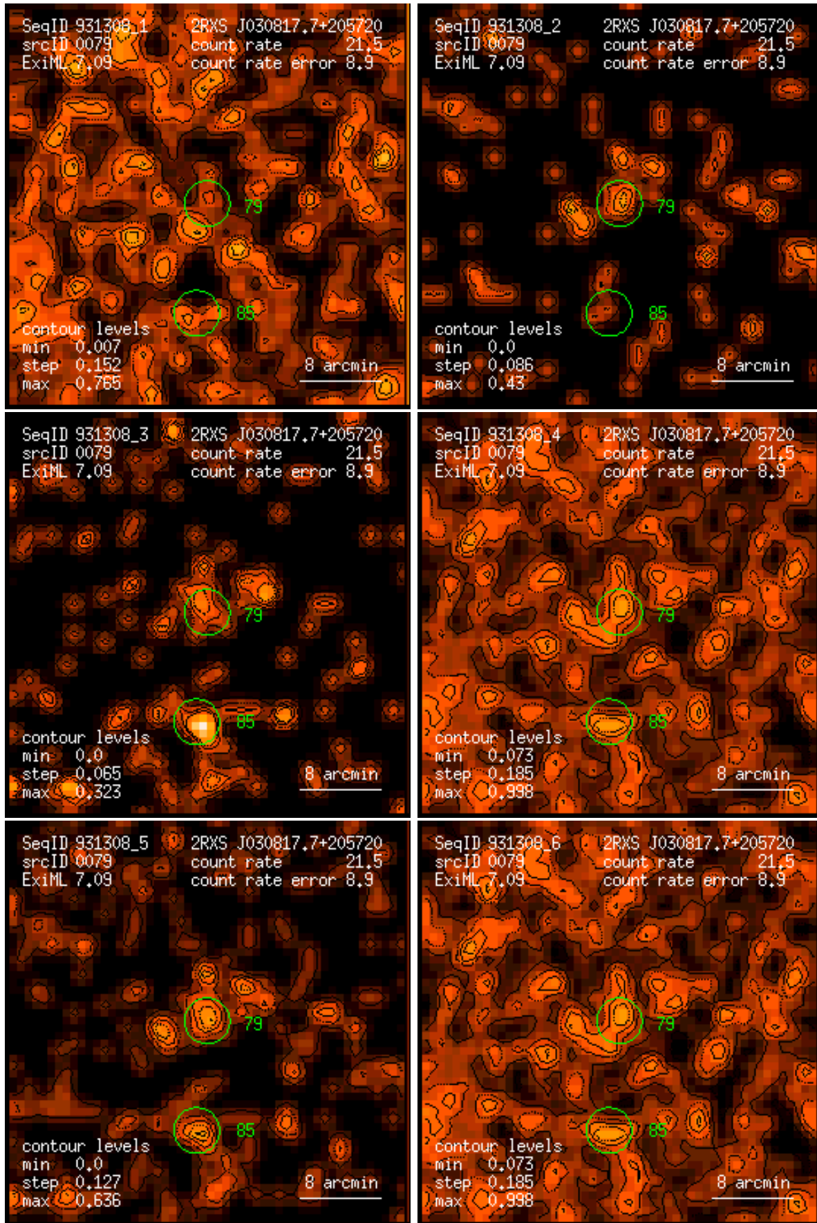
Figure 79: RASS 931308: detection 0079: band rate images, Gaussian filter: (1) PSPC channels 11 – 41, (2) 52 – 90, (3) 91 – 201, (4) 11 – 235, (5) 52 – 201, (6) 11 – 201. Broad band rates in counts/ks. Band rate contour levels in counts/ks/arcmin 2 .
