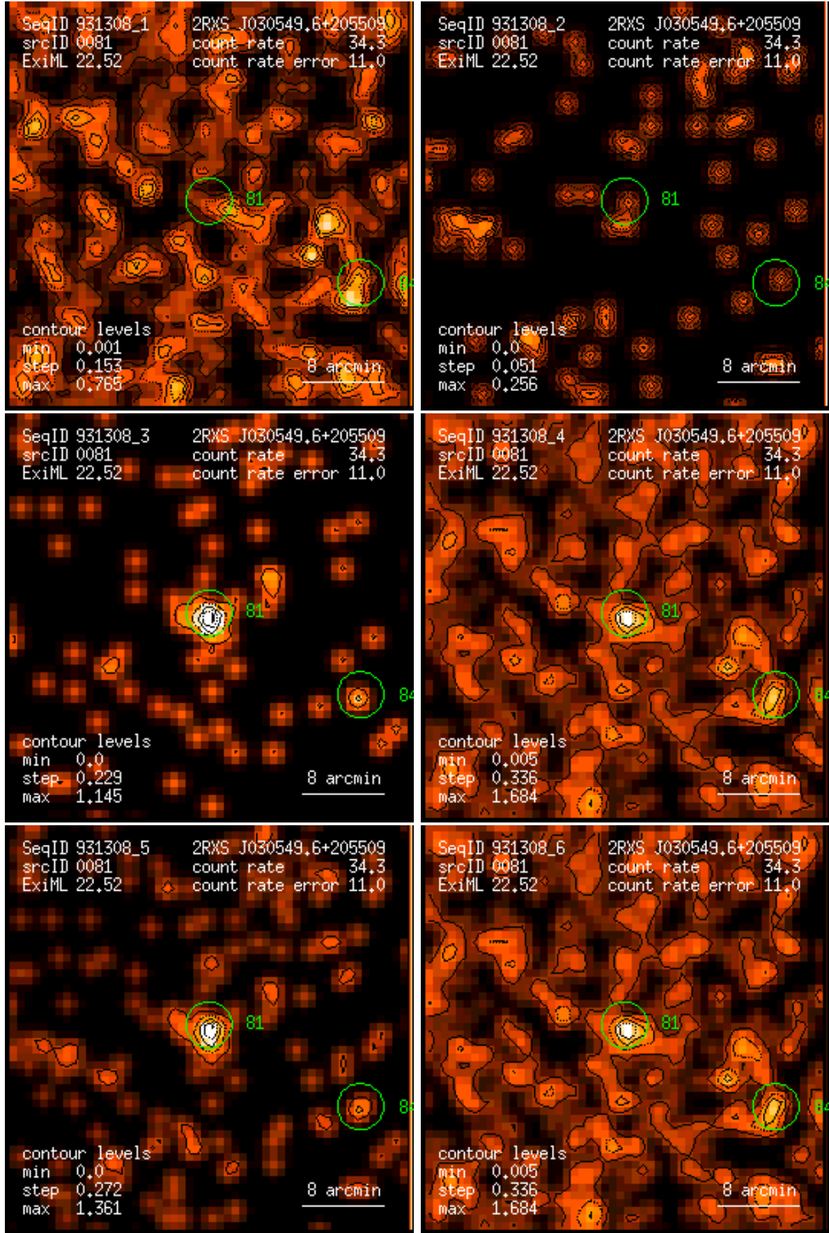
Figure 81: RASS 931308: detection 0081: band rate images, Gaussian filter: (1) PSPC channels 11 – 41, (2) 52 – 90, (3) 91 – 201, (4) 11 – 235, (5) 52 – 201, (6) 11 – 201. Broad band rates in counts/ks. Band rate contour levels in counts/ks/arcmin 2 .
