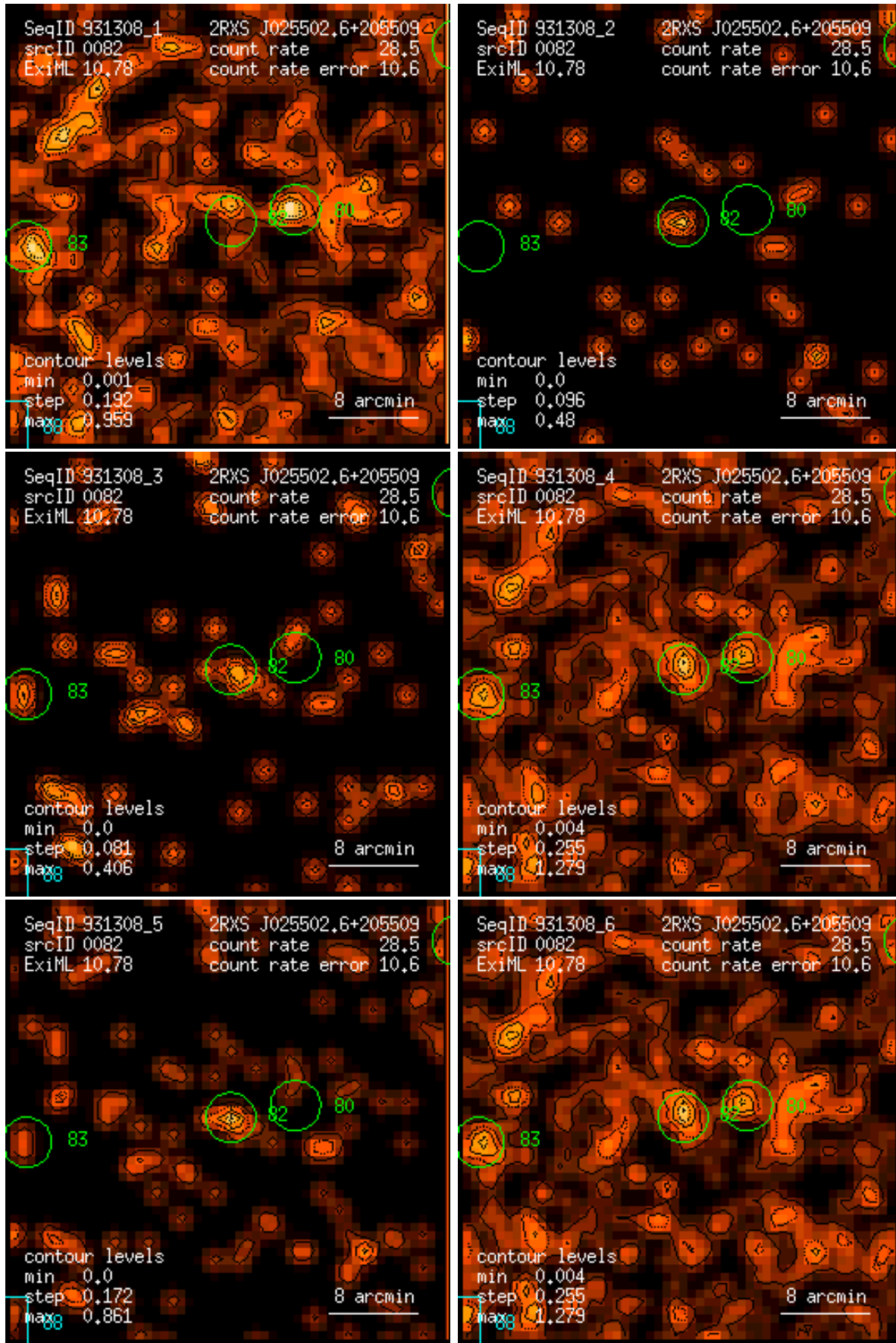
Figure 82: RASS 931308: detection 0082: band rate images, Gaussian filter: (1) PSPC channels 11 – 41, (2) 52 – 90, (3) 91 – 201, (4) 11 – 235, (5) 52 – 201, (6) 11 – 201. Broad band rates in counts/ks. Band rate contour levels in counts/ks/arcmin 2 .
