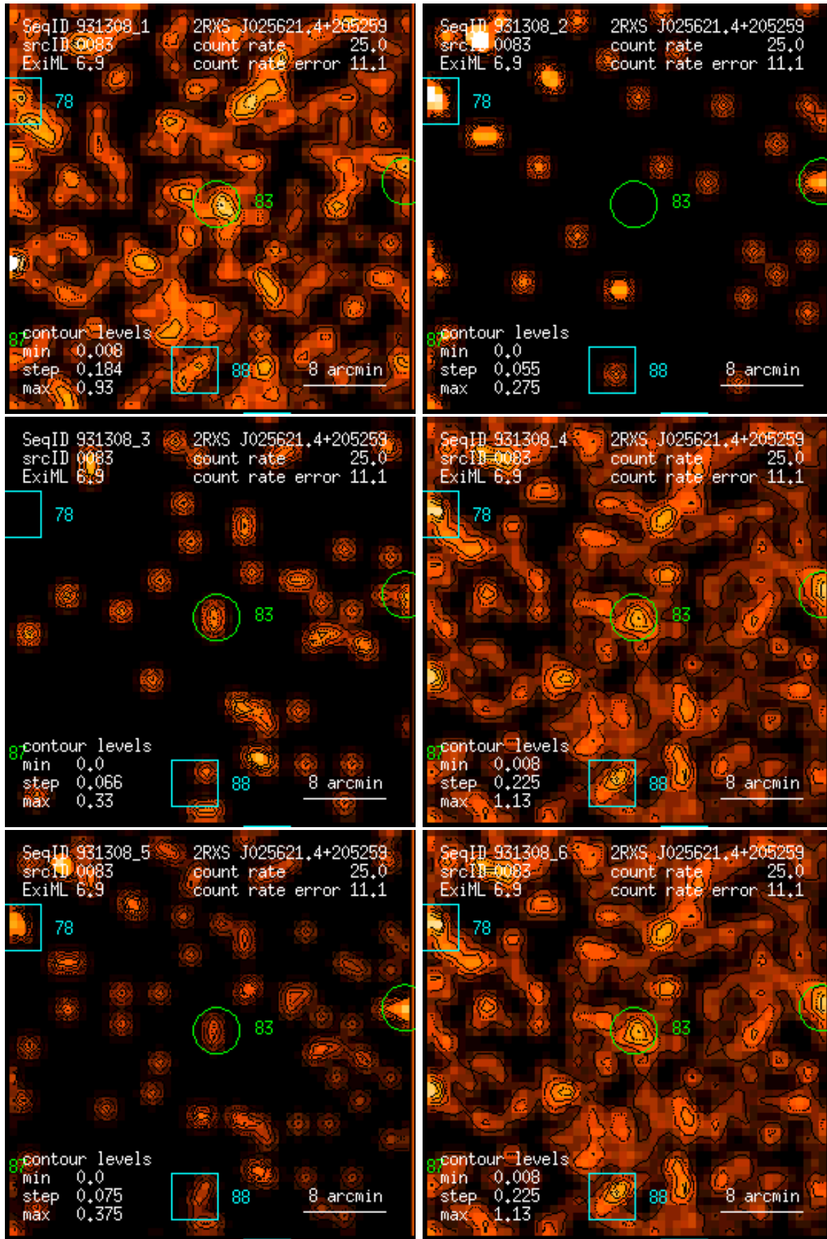
Figure 83: RASS 931308: detection 0083: band rate images, Gaussian filter: (1) PSPC channels 11 – 41, (2) 52 – 90, (3) 91 – 201, (4) 11 – 235, (5) 52 – 201, (6) 11 – 201. Broad band rates in counts/ks. Band rate contour levels in counts/ks/arcmin 2 .
