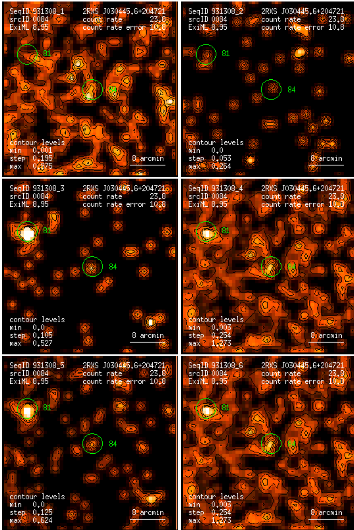
Figure 84: RASS 931308: detection 0084: band rate images, Gaussian filter: (1) PSPC channels 11 – 41, (2) 52 – 90, (3) 91 – 201, (4) 11 – 235, (5) 52 – 201, (6) 11 – 201. Broad band rates in counts/ks. Band rate contour levels in counts/ks/arcmin 2 .
