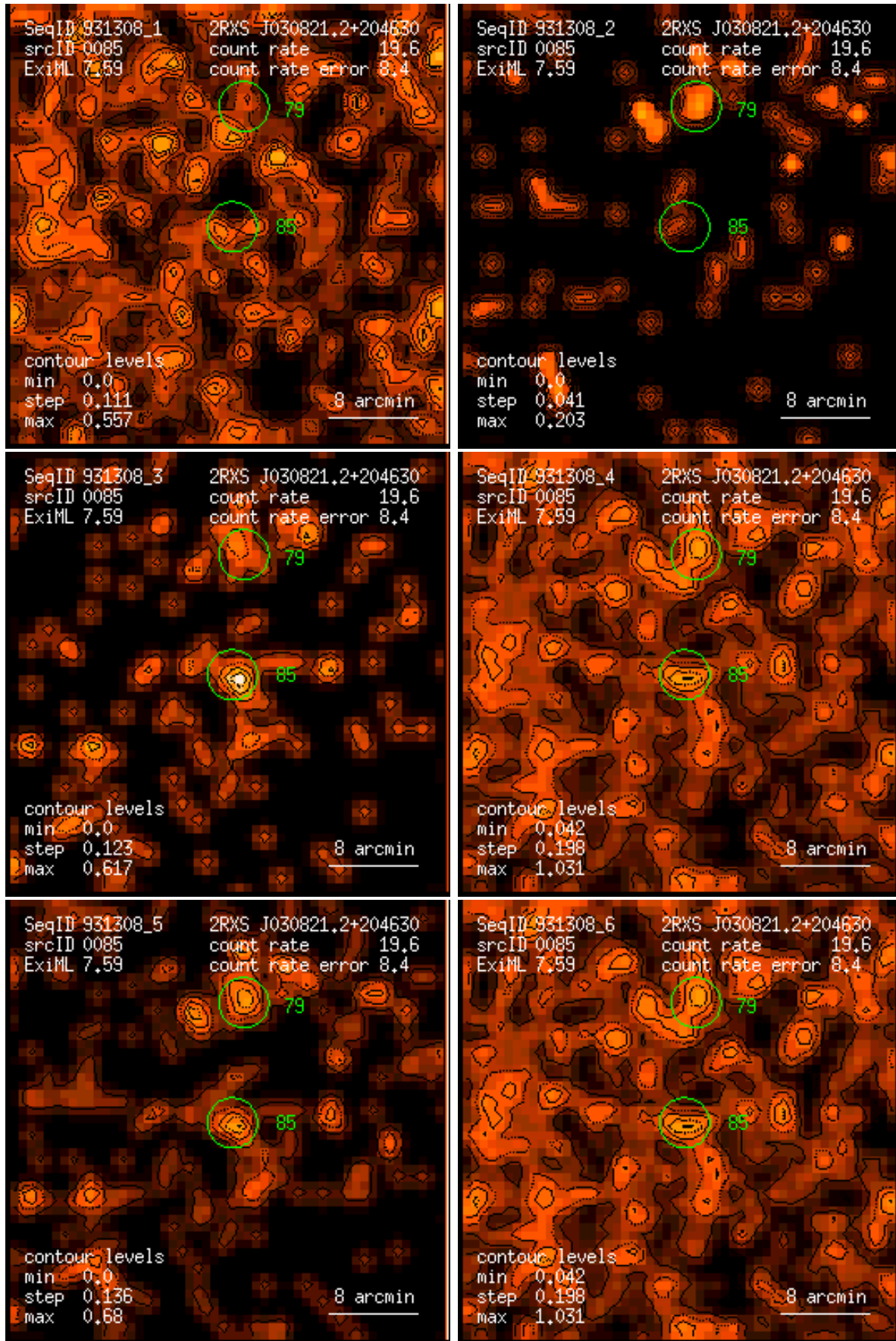
Figure 85: RASS 931308: detection 0085: band rate images, Gaussian filter: (1) PSPC channels 11 – 41, (2) 52 – 90, (3) 91 – 201, (4) 11 – 235, (5) 52 – 201, (6) 11 – 201. Broad band rates in counts/ks. Band rate contour levels in counts/ks/arcmin 2 .
