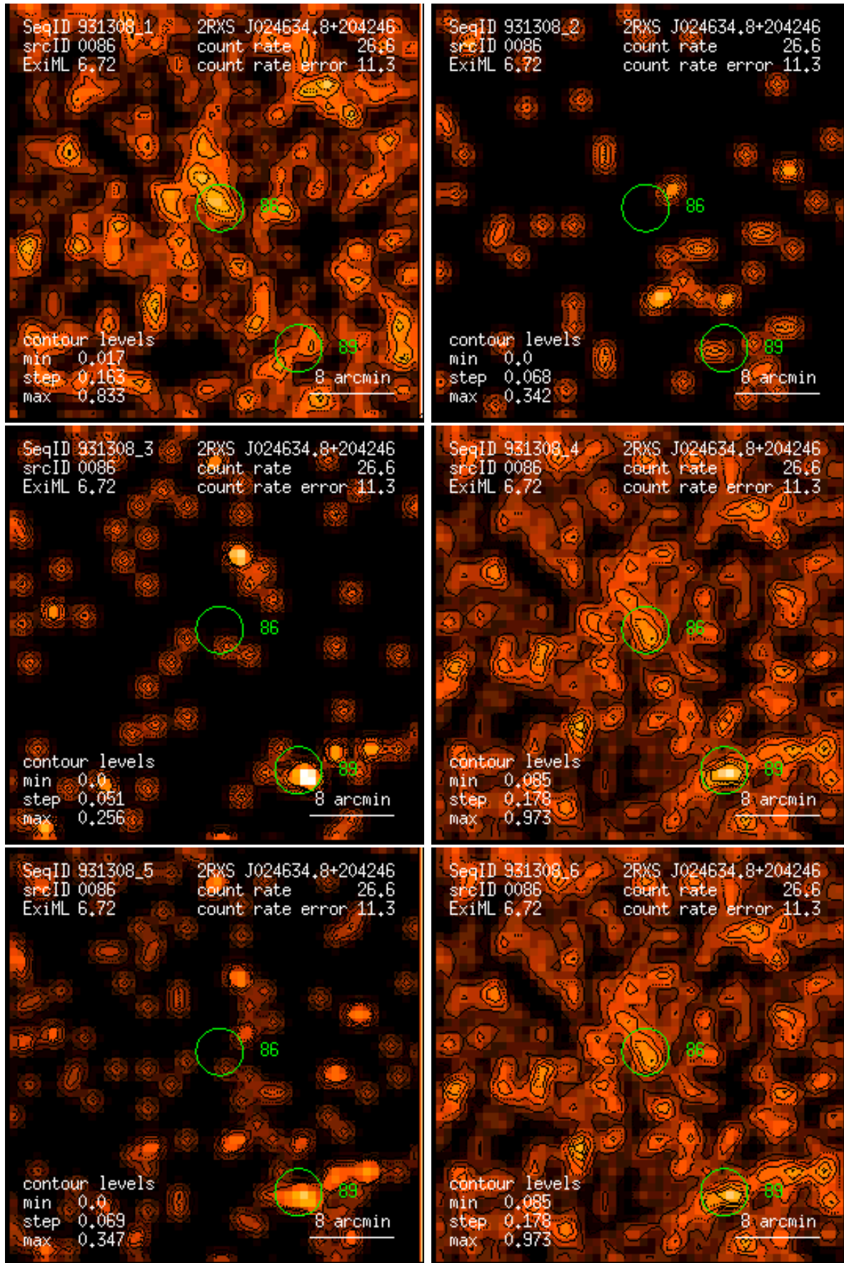
Figure 86: RASS 931308: detection 0086: band rate images, Gaussian filter: (1) PSPC channels 11 – 41, (2) 52 – 90, (3) 91 – 201, (4) 11 – 235, (5) 52 – 201, (6) 11 – 201. Broad band rates in counts/ks. Band rate contour levels in counts/ks/arcmin 2 .
