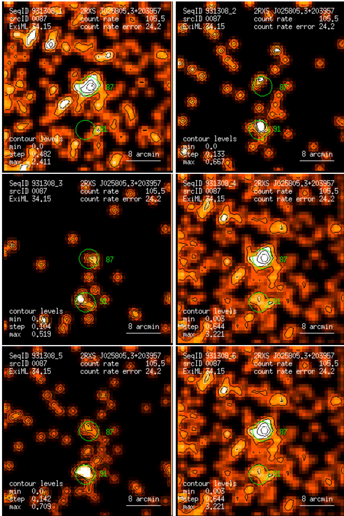
Figure 87: RASS 931308: detection 0087: band rate images, Gaussian filter: (1) PSPC channels 11 – 41, (2) 52 – 90, (3) 91 – 201, (4) 11 – 235, (5) 52 – 201, (6) 11 – 201. Broad band rates in counts/ks. Band rate contour levels in counts/ks/arcmin 2 .
