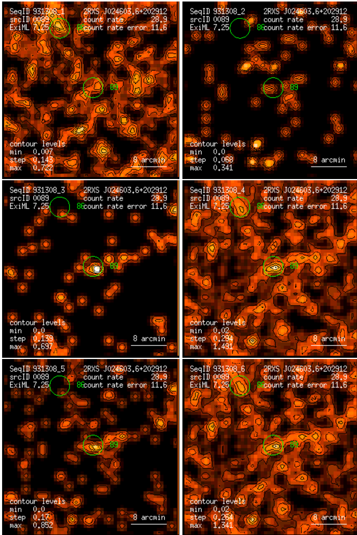
Figure 89: RASS 931308: detection 0089: band rate images, Gaussian filter: (1) PSPC channels 11 – 41, (2) 52 – 90, (3) 91 – 201, (4) 11 – 235, (5) 52 – 201, (6) 11 – 201. Broad band rates in counts/ks. Band rate contour levels in counts/ks/arcmin 2 .
