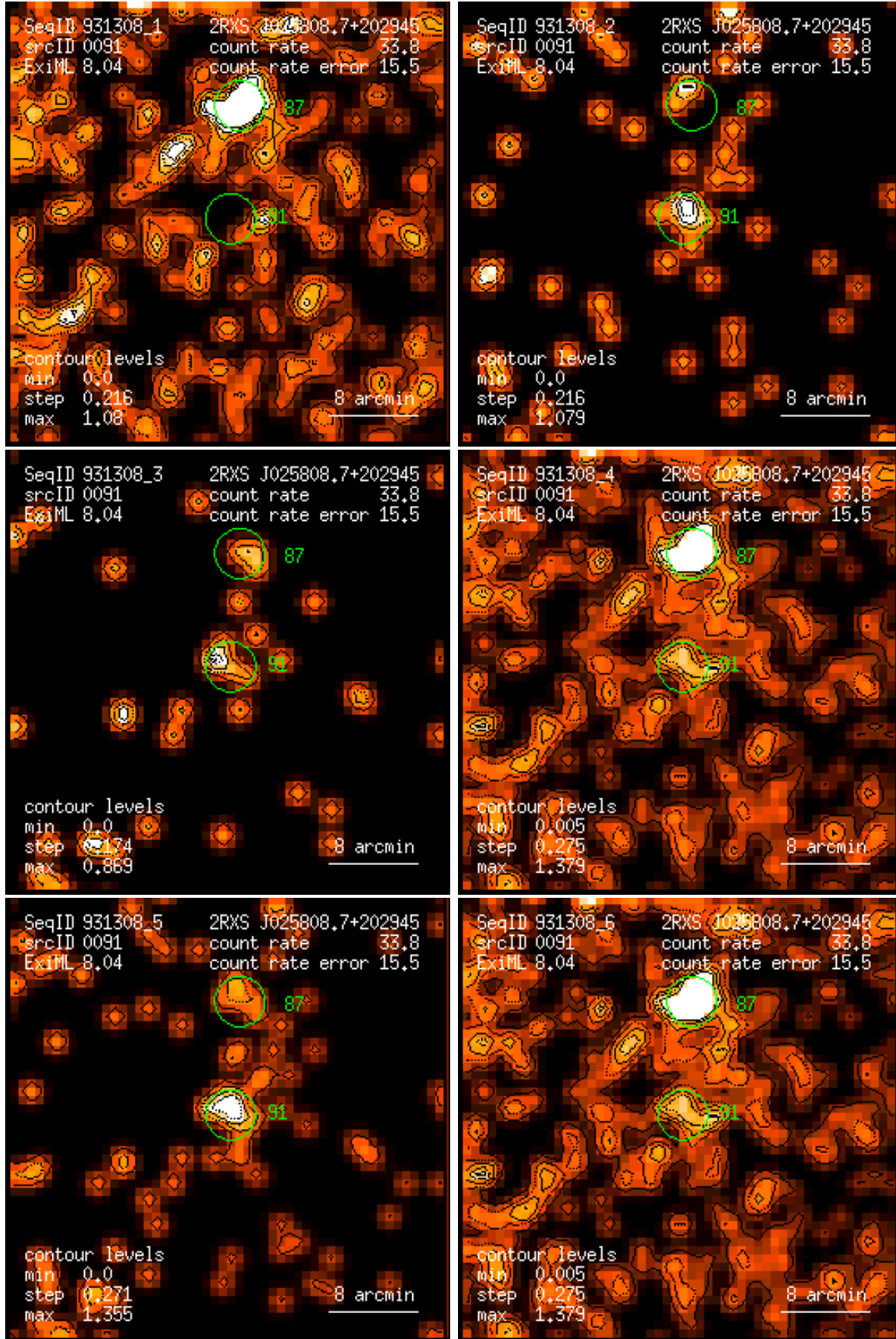
Figure 91: RASS 931308: detection 0091: band rate images, Gaussian filter: (1) PSPC channels 11 – 41, (2) 52 – 90, (3) 91 – 201, (4) 11 – 235, (5) 52 – 201, (6) 11 – 201. Broad band rates in counts/ks. Band rate contour levels in counts/ks/arcmin 2 .
