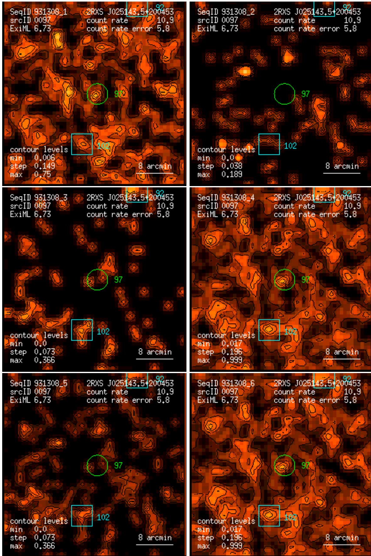
Figure 97: RASS 931308: detection 0097: band rate images, Gaussian filter: (1) PSPC channels 11 – 41, (2) 52 – 90, (3) 91 – 201, (4) 11 – 235, (5) 52 – 201, (6) 11 – 201. Broad band rates in counts/ks. Band rate contour levels in counts/ks/arcmin 2 .
