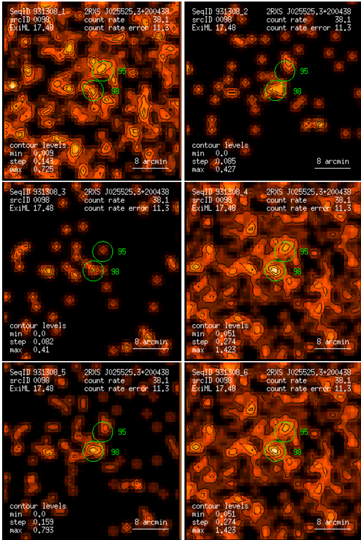
Figure 98: RASS 931308: detection 0098: band rate images, Gaussian filter: (1) PSPC channels 11 – 41, (2) 52 – 90, (3) 91 – 201, (4) 11 – 235, (5) 52 – 201, (6) 11 – 201. Broad band rates in counts/ks. Band rate contour levels in counts/ks/arcmin 2 .
