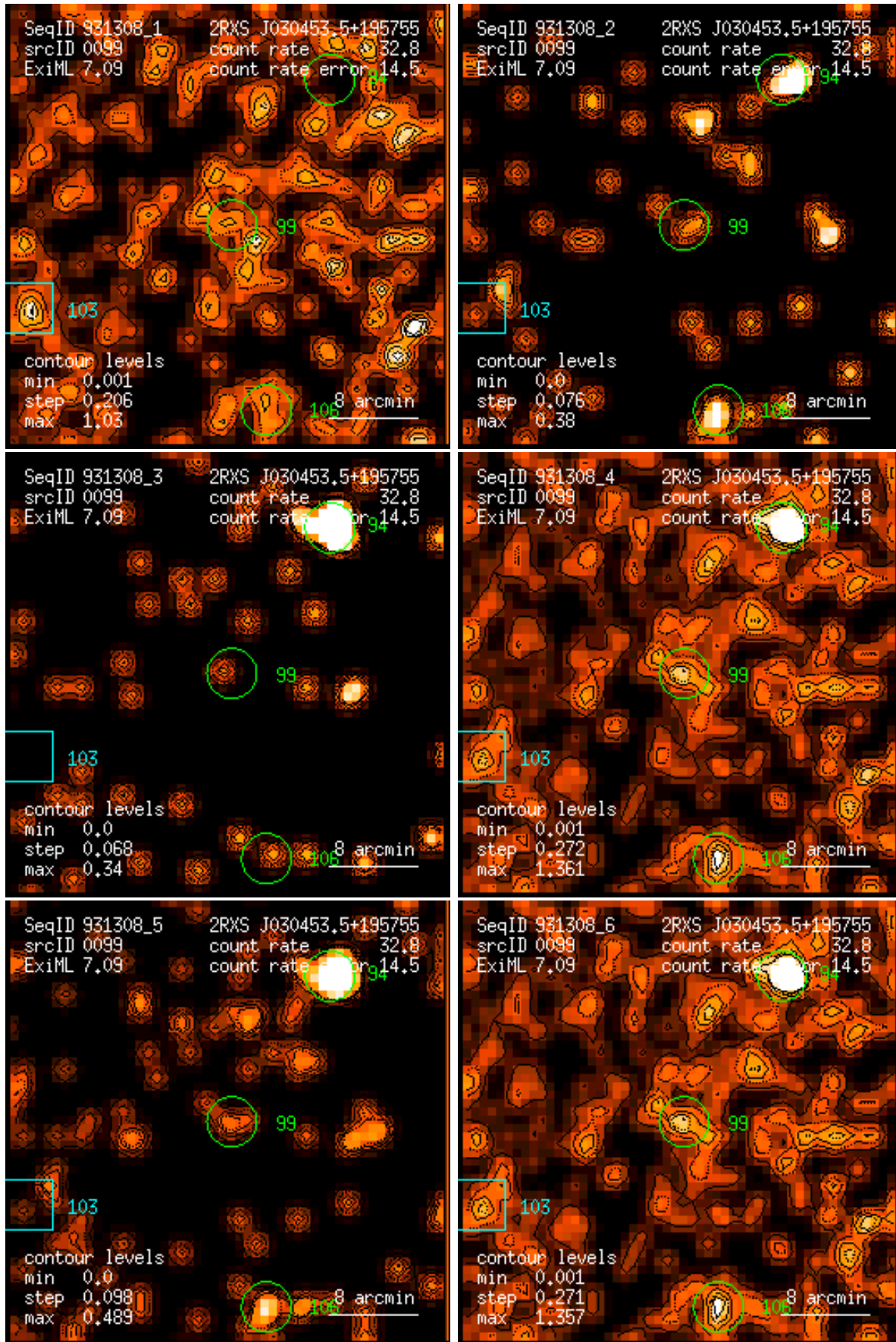
Figure 99: RASS 931308: detection 0099: band rate images, Gaussian filter: (1) PSPC channels 11 – 41, (2) 52 – 90, (3) 91 – 201, (4) 11 – 235, (5) 52 – 201, (6) 11 – 201. Broad band rates in counts/ks. Band rate contour levels in counts/ks/arcmin 2 .
