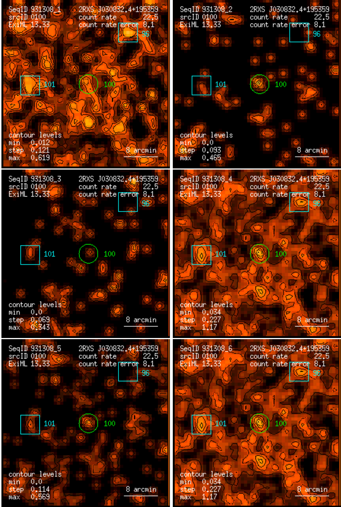
Figure 100: RASS 931308: detection 0100: band rate images, Gaussian filter: (1) PSPC channels 11 – 41, (2) 52 – 90, (3) 91 – 201, (4) 11 – 235, (5) 52 – 201, (6) 11 – 201. Broad band rates in counts/ks. Band rate contour levels in counts/ks/arcmin 2 .
