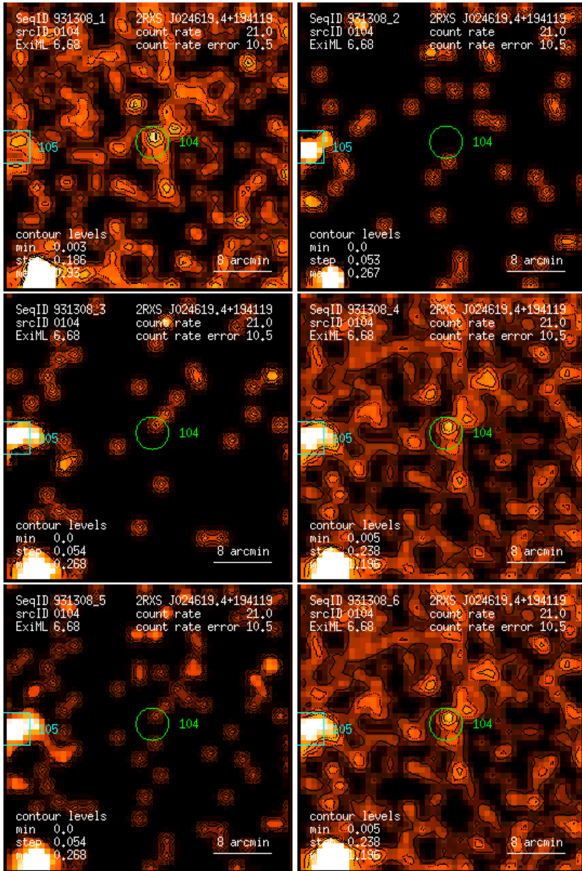
Figure 104: RASS 931308: detection 0104: band rate images, Gaussian filter: (1) PSPC channels 11 – 41, (2) 52 – 90, (3) 91 – 201, (4) 11 – 235, (5) 52 – 201, (6) 11 – 201. Broad band rates in counts/ks. Band rate contour levels in counts/ks/arcmin 2 .
