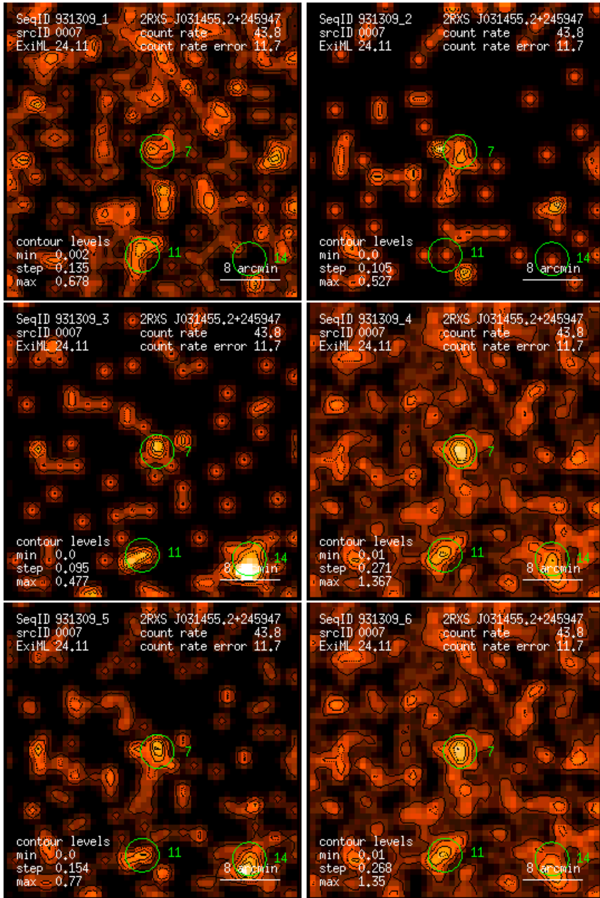
Figure 7: RASS 931309: detection 0007: band rate images, Gaussian filter: (1) PSPC channels 11 – 41, (2) 52 – 90, (3) 91 – 201, (4) 11 – 235, (5) 52 – 201, (6) 11 – 201. Broad band rates in counts/ks. Band rate contour levels in counts/ks/arcmin 2 .
