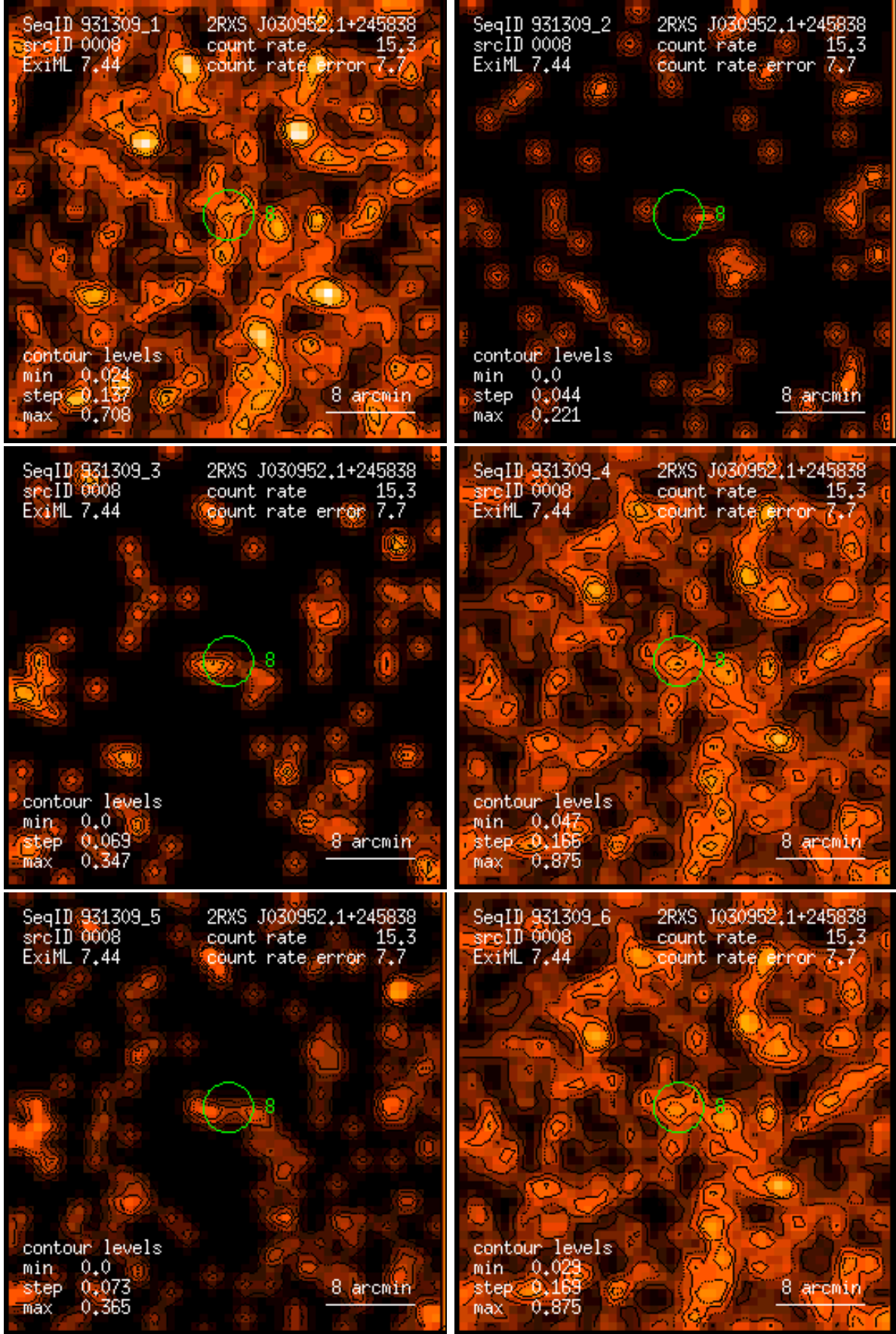
Figure 8: RASS 931309: detection 0008: band rate images, Gaussian filter: (1) PSPC channels 11 – 41, (2) 52 – 90, (3) 91 – 201, (4) 11 – 235, (5) 52 – 201, (6) 11 – 201. Broad band rates in counts/ks. Band rate contour levels in counts/ks/arcmin 2 .
