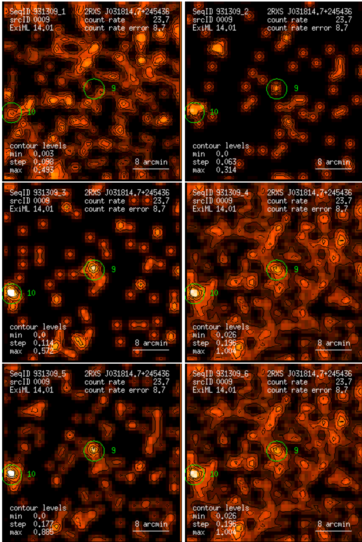
Figure 9: RASS 931309: detection 0009: band rate images, Gaussian filter: (1) PSPC channels 11 – 41, (2) 52 – 90, (3) 91 – 201, (4) 11 – 235, (5) 52 – 201, (6) 11 – 201. Broad band rates in counts/ks. Band rate contour levels in counts/ks/arcmin 2 .
