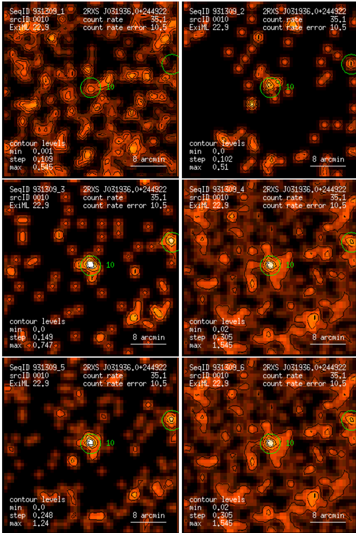
Figure 10: RASS 931309: detection 0010: band rate images, Gaussian filter: (1) PSPC channels 11 – 41, (2) 52 – 90, (3) 91 – 201, (4) 11 – 235, (5) 52 – 201, (6) 11 – 201. Broad band rates in counts/ks. Band rate contour levels in counts/ks/arcmin 2 .
