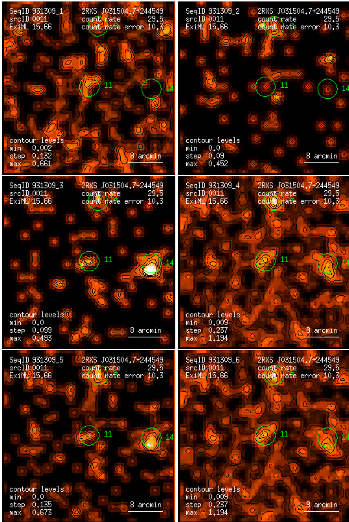
Figure 11: RASS 931309: detection 0011: band rate images, Gaussian filter: (1) PSPC channels 11 – 41, (2) 52 – 90, (3) 91 – 201, (4) 11 – 235, (5) 52 – 201, (6) 11 – 201. Broad band rates in counts/ks. Band rate contour levels in counts/ks/arcmin 2 .
