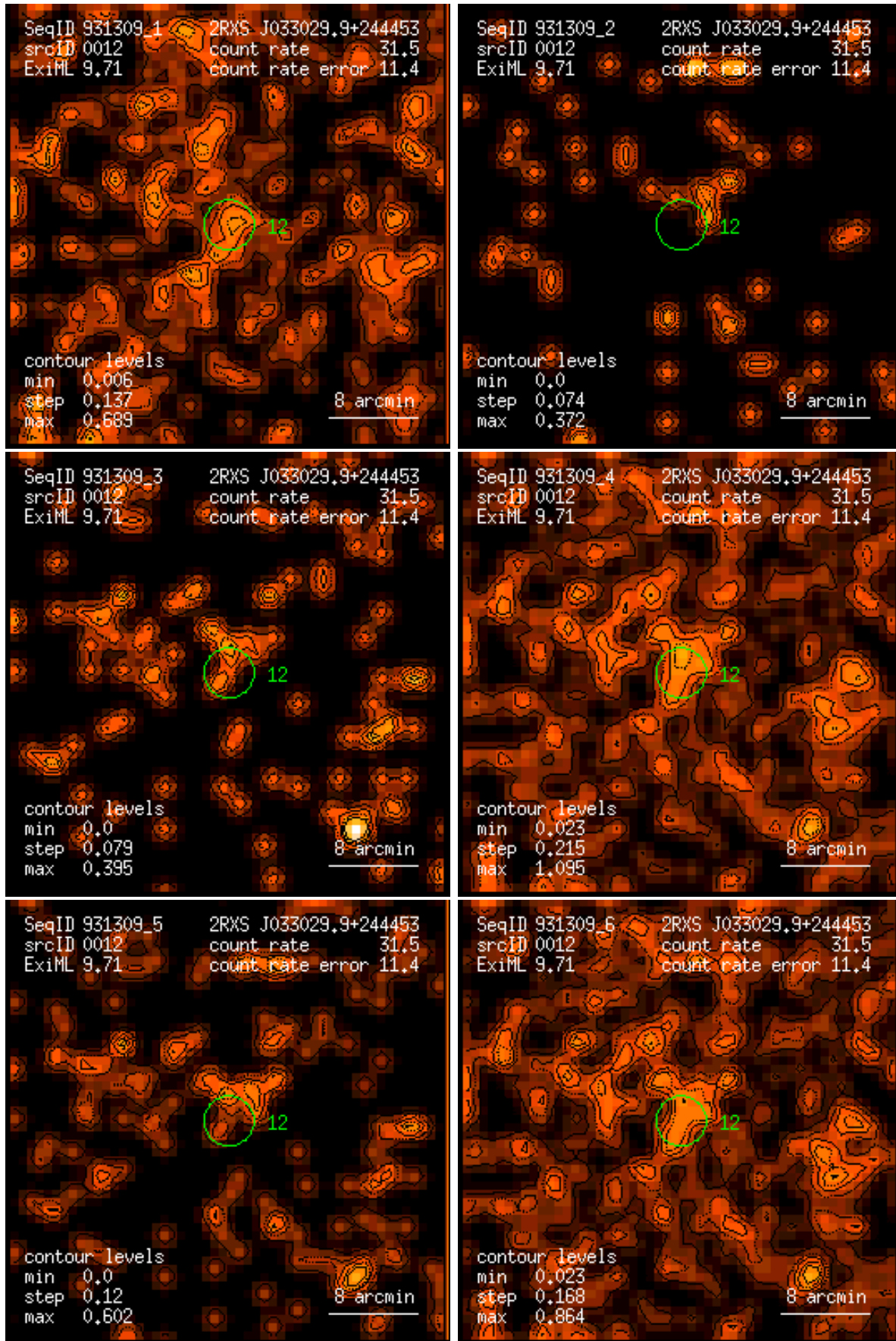
Figure 12: RASS 931309: detection 0012: band rate images, Gaussian filter: (1) PSPC channels 11 – 41, (2) 52 – 90, (3) 91 – 201, (4) 11 – 235, (5) 52 – 201, (6) 11 – 201. Broad band rates in counts/ks. Band rate contour levels in counts/ks/arcmin 2 .
