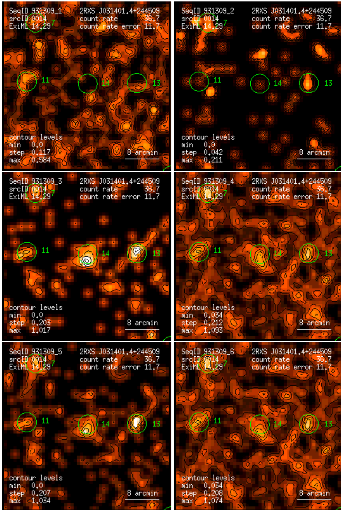
Figure 14: RASS 931309: detection 0014: band rate images, Gaussian filter: (1) PSPC channels 11 – 41, (2) 52 – 90, (3) 91 – 201, (4) 11 – 235, (5) 52 – 201, (6) 11 – 201. Broad band rates in counts/ks. Band rate contour levels in counts/ks/arcmin 2 .
