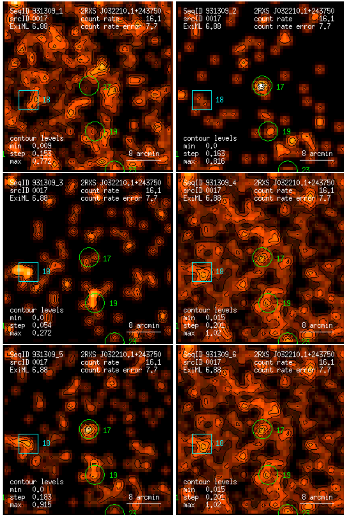
Figure 17: RASS 931309: detection 0017: band rate images, Gaussian filter: (1) PSPC channels 11 – 41, (2) 52 – 90, (3) 91 – 201, (4) 11 – 235, (5) 52 – 201, (6) 11 – 201. Broad band rates in counts/ks. Band rate contour levels in counts/ks/arcmin 2 .
