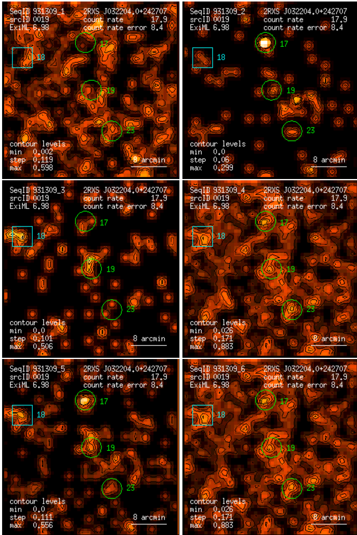
Figure 19: RASS 931309: detection 0019: band rate images, Gaussian filter: (1) PSPC channels 11 – 41, (2) 52 – 90, (3) 91 – 201, (4) 11 – 235, (5) 52 – 201, (6) 11 – 201. Broad band rates in counts/ks. Band rate contour levels in counts/ks/arcmin 2 .
