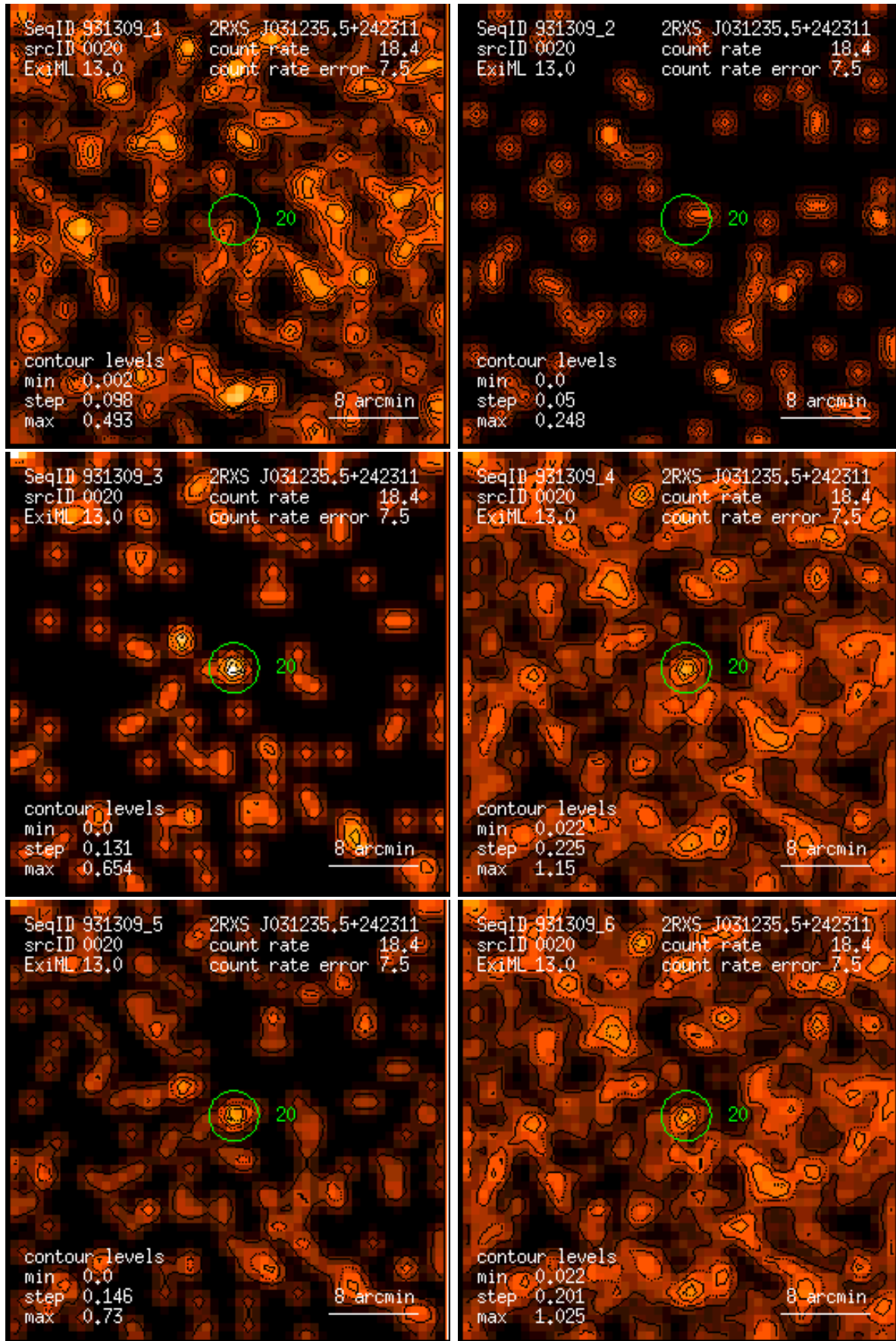
Figure 20: RASS 931309: detection 0020: band rate images, Gaussian filter: (1) PSPC channels 11 – 41, (2) 52 – 90, (3) 91 – 201, (4) 11 – 235, (5) 52 – 201, (6) 11 – 201. Broad band rates in counts/ks. Band rate contour levels in counts/ks/arcmin 2 .
