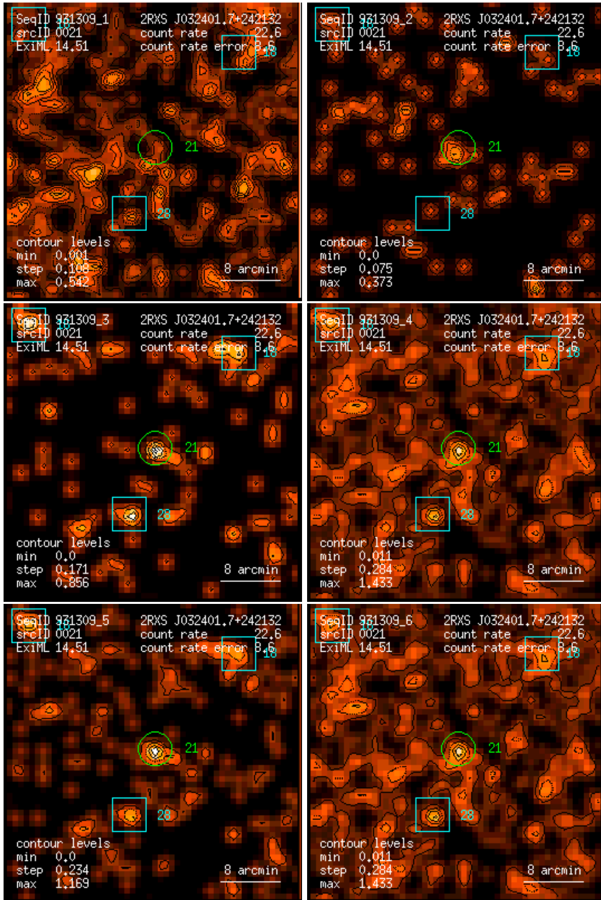
Figure 21: RASS 931309: detection 0021: band rate images, Gaussian filter: (1) PSPC channels 11 – 41, (2) 52 – 90, (3) 91 – 201, (4) 11 – 235, (5) 52 – 201, (6) 11 – 201. Broad band rates in counts/ks. Band rate contour levels in counts/ks/arcmin 2 .
