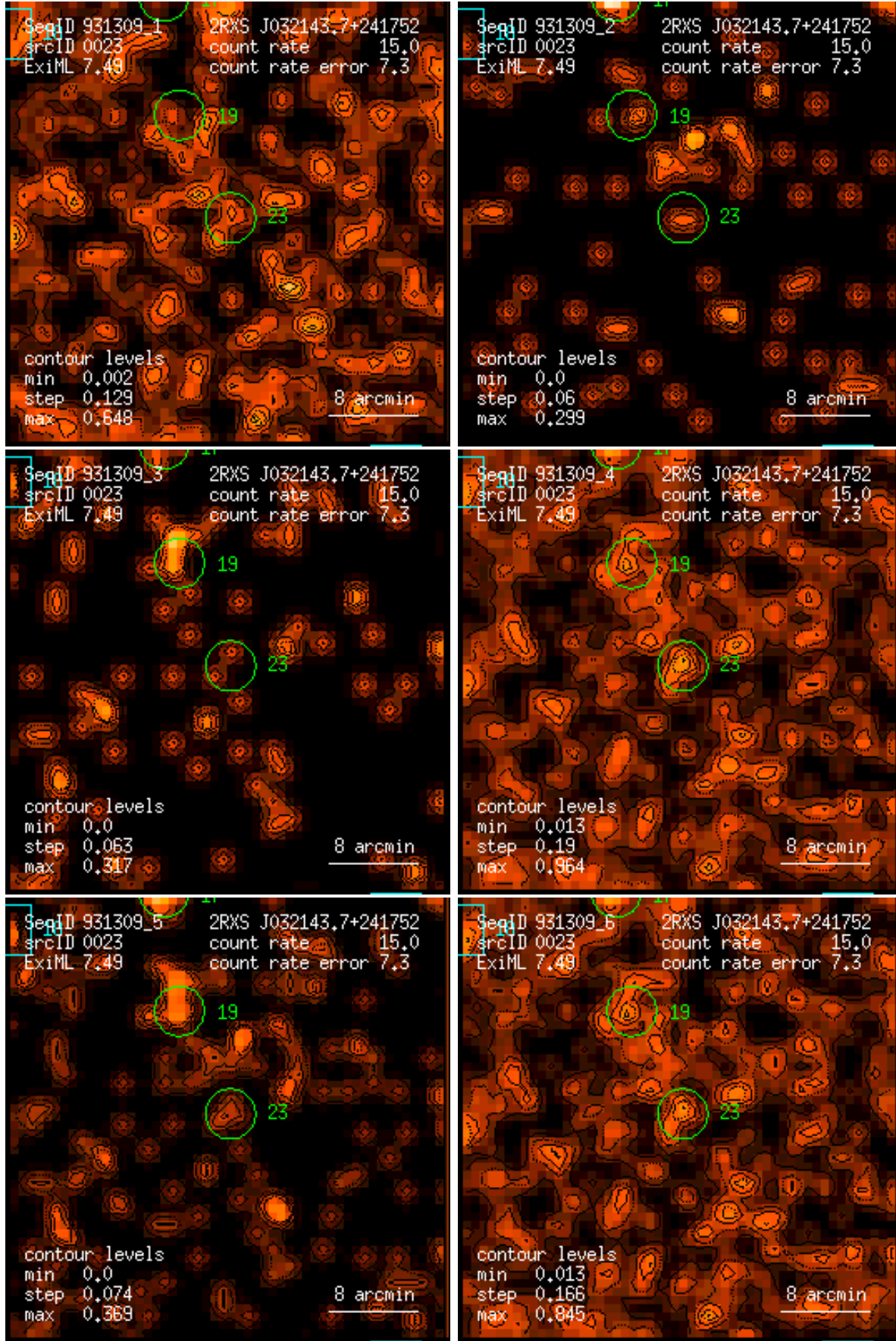
Figure 23: RASS 931309: detection 0023: band rate images, Gaussian filter: (1) PSPC channels 11 – 41, (2) 52 – 90, (3) 91 – 201, (4) 11 – 235, (5) 52 – 201, (6) 11 – 201. Broad band rates in counts/ks. Band rate contour levels in counts/ks/arcmin 2 .
