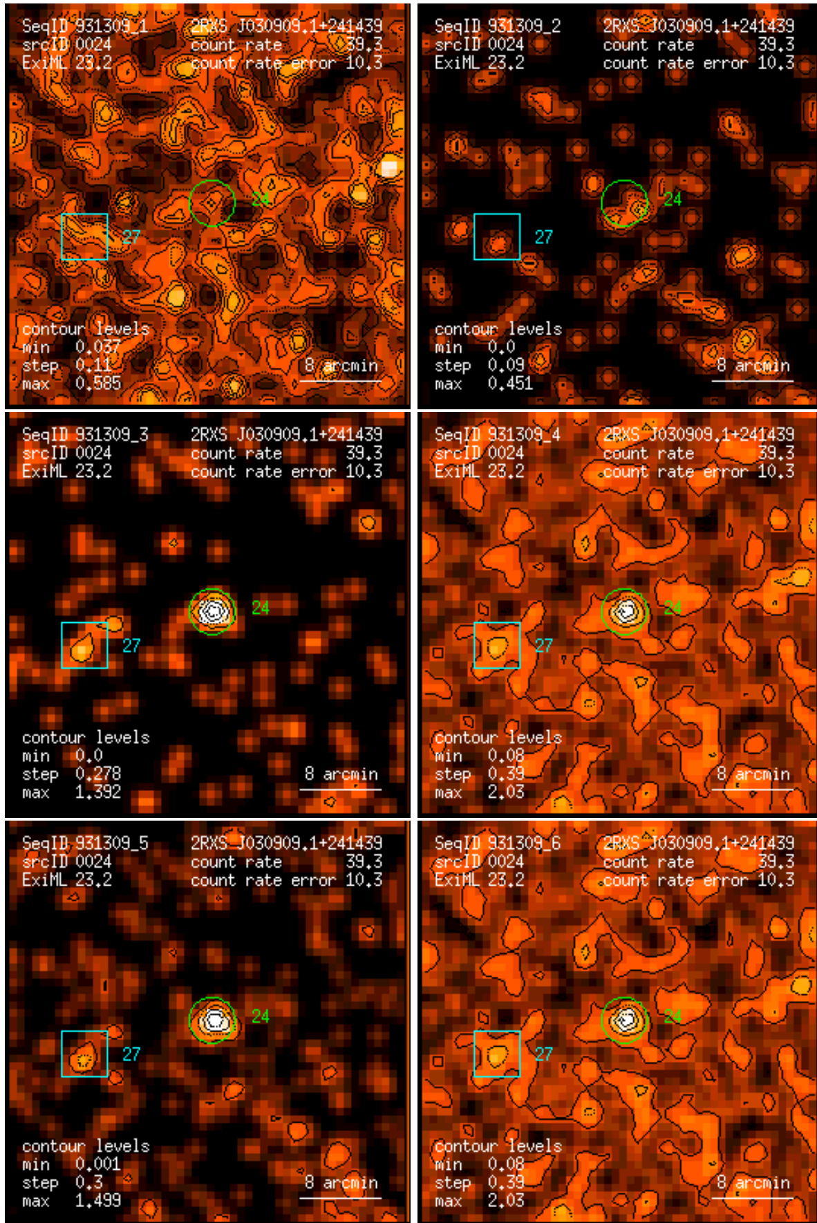
Figure 24: RASS 931309: detection 0024: band rate images, Gaussian filter: (1) PSPC channels 11 – 41, (2) 52 – 90, (3) 91 – 201, (4) 11 – 235, (5) 52 – 201, (6) 11 – 201. Broad band rates in counts/ks. Band rate contour levels in counts/ks/arcmin 2 .
