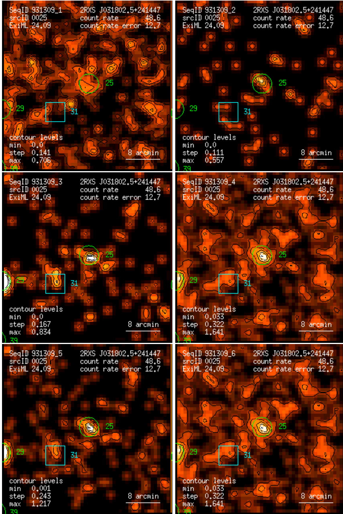
Figure 25: RASS 931309: detection 0025: band rate images, Gaussian filter: (1) PSPC channels 11 – 41, (2) 52 – 90, (3) 91 – 201, (4) 11 – 235, (5) 52 – 201, (6) 11 – 201. Broad band rates in counts/ks. Band rate contour levels in counts/ks/arcmin 2 .
