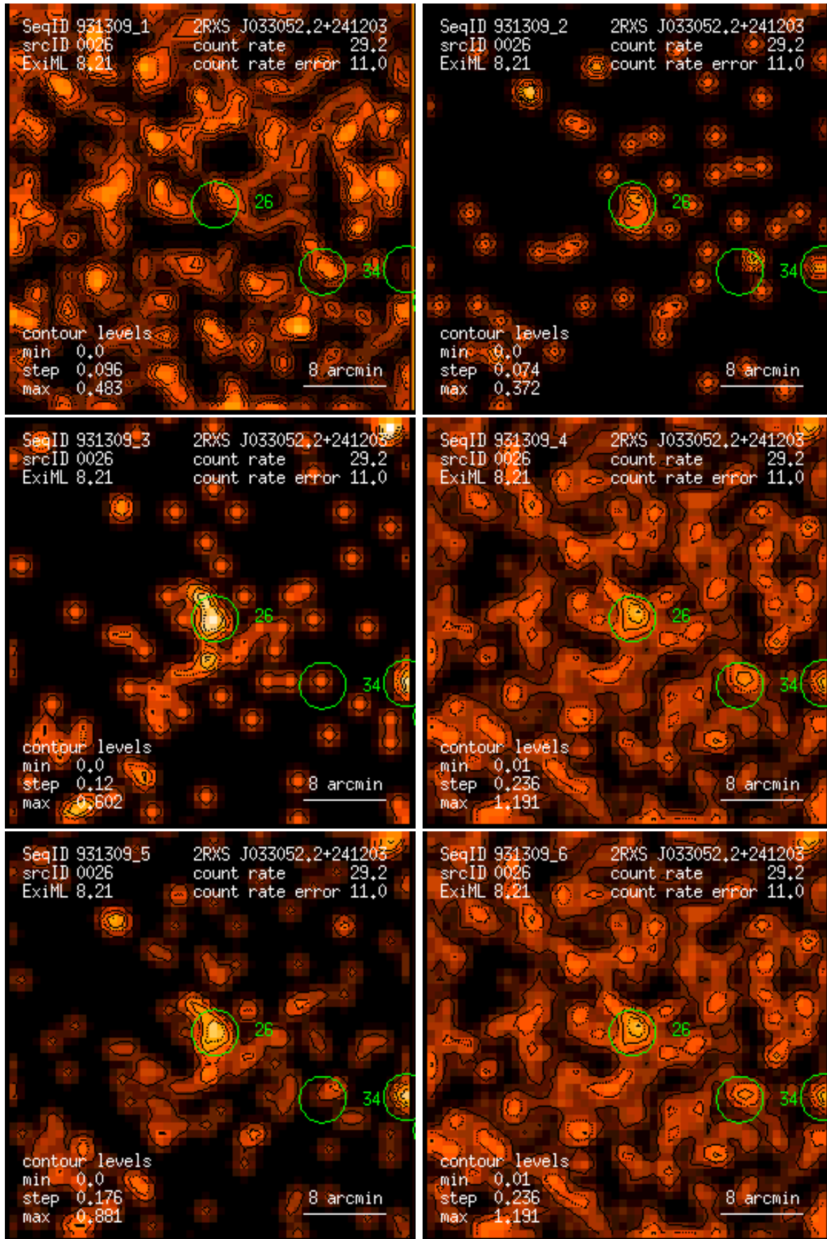
Figure 26: RASS 931309: detection 0026: band rate images, Gaussian filter: (1) PSPC channels 11 – 41, (2) 52 – 90, (3) 91 – 201, (4) 11 – 235, (5) 52 – 201, (6) 11 – 201. Broad band rates in counts/ks. Band rate contour levels in counts/ks/arcmin 2 .
