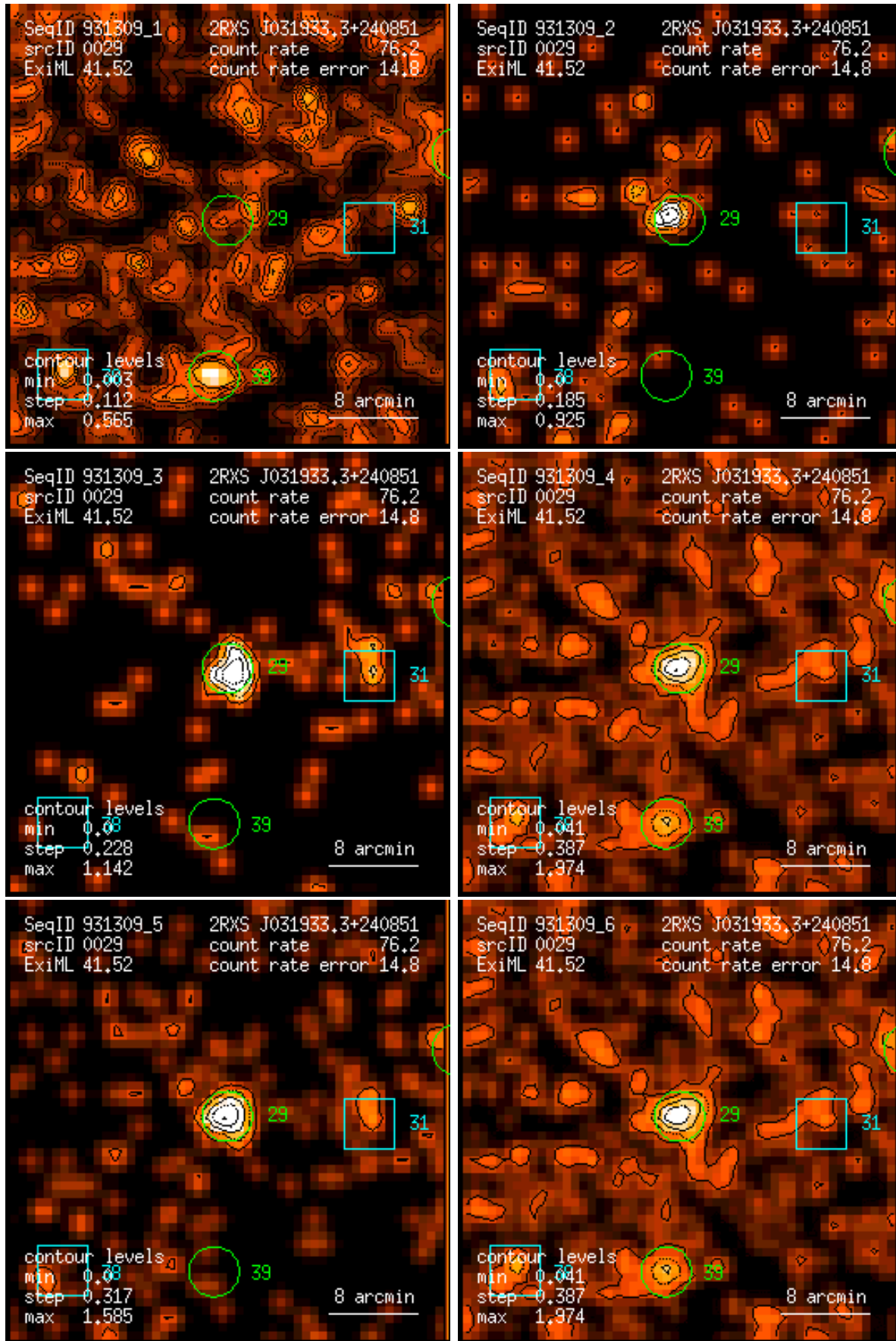
Figure 29: RASS 931309: detection 0029: band rate images, Gaussian filter: (1) PSPC channels 11 – 41, (2) 52 – 90, (3) 91 – 201, (4) 11 – 235, (5) 52 – 201, (6) 11 – 201. Broad band rates in counts/ks. Band rate contour levels in counts/ks/arcmin 2 .
