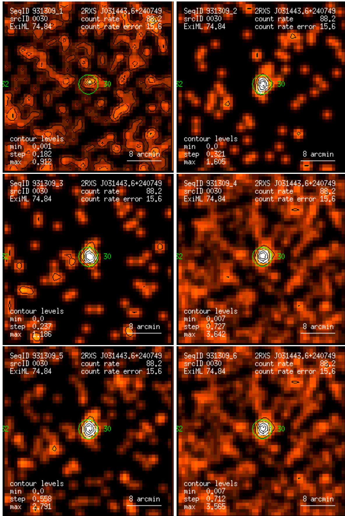
Figure 30: RASS 931309: detection 0030: band rate images, Gaussian filter: (1) PSPC channels 11 – 41, (2) 52 – 90, (3) 91 – 201, (4) 11 – 235, (5) 52 – 201, (6) 11 – 201. Broad band rates in counts/ks. Band rate contour levels in counts/ks/arcmin 2 .
