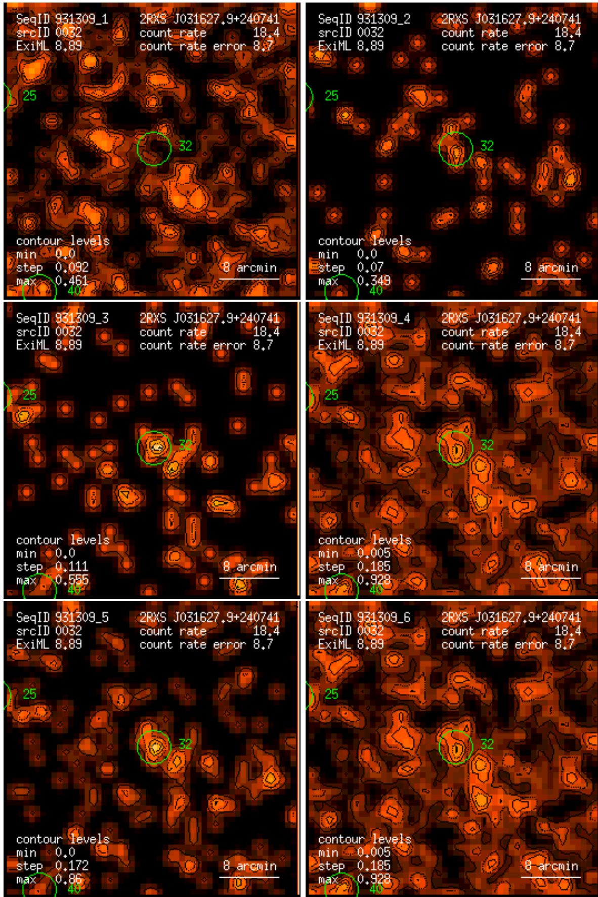
Figure 32: RASS 931309: detection 0032: band rate images, Gaussian filter: (1) PSPC channels 11 – 41, (2) 52 – 90, (3) 91 – 201, (4) 11 – 235, (5) 52 – 201, (6) 11 – 201. Broad band rates in counts/ks. Band rate contour levels in counts/ks/arcmin 2 .
