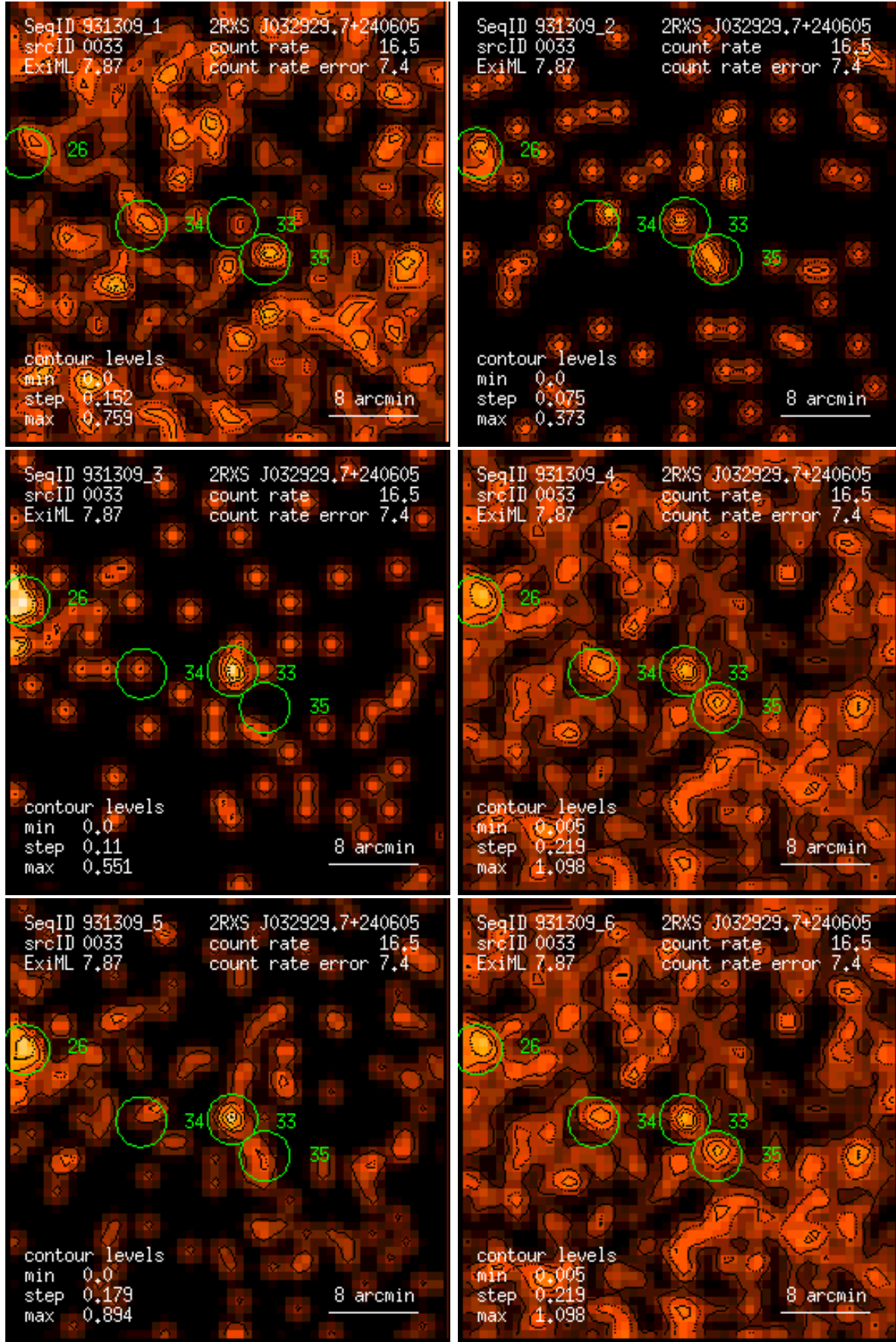
Figure 33: RASS 931309: detection 0033: band rate images, Gaussian filter: (1) PSPC channels 11 – 41, (2) 52 – 90, (3) 91 – 201, (4) 11 – 235, (5) 52 – 201, (6) 11 – 201. Broad band rates in counts/ks. Band rate contour levels in counts/ks/arcmin 2 .
