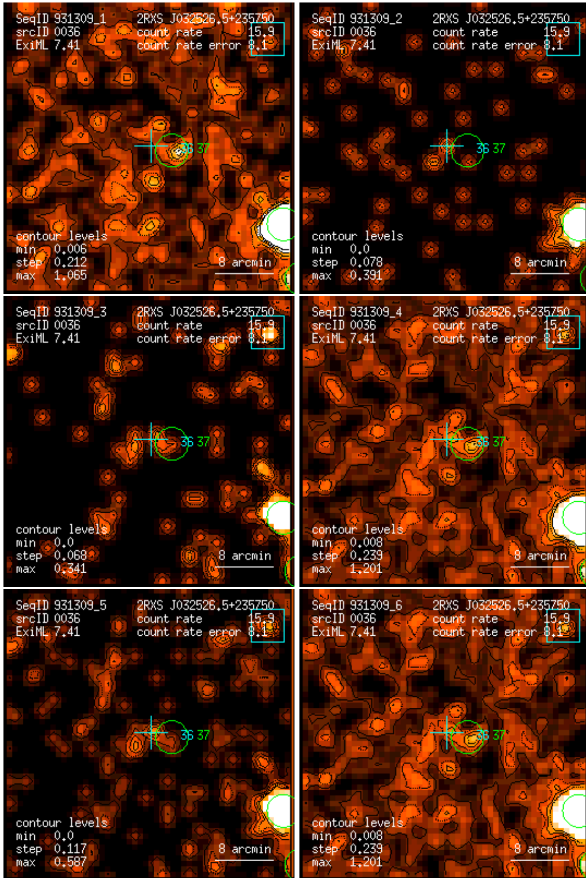
Figure 36: RASS 931309: detection 0036: band rate images, Gaussian filter: (1) PSPC channels 11 – 41, (2) 52 – 90, (3) 91 – 201, (4) 11 – 235, (5) 52 – 201, (6) 11 – 201. Broad band rates in counts/ks. Band rate contour levels in counts/ks/arcmin 2 .
