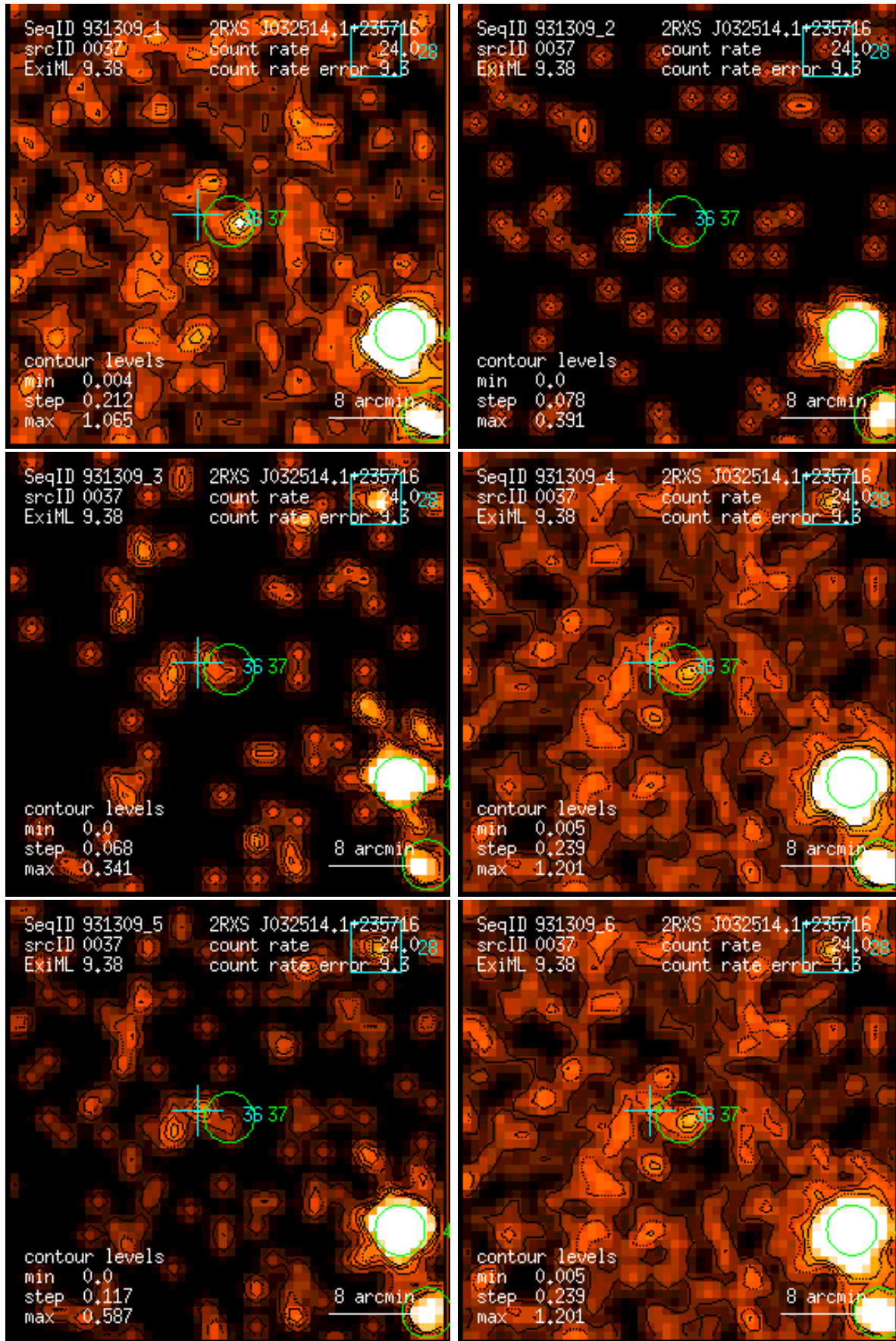
Figure 37: RASS 931309: detection 0037: band rate images, Gaussian filter: (1) PSPC channels 11 – 41, (2) 52 – 90, (3) 91 – 201, (4) 11 – 235, (5) 52 – 201, (6) 11 – 201. Broad band rates in counts/ks. Band rate contour levels in counts/ks/arcmin 2 .
