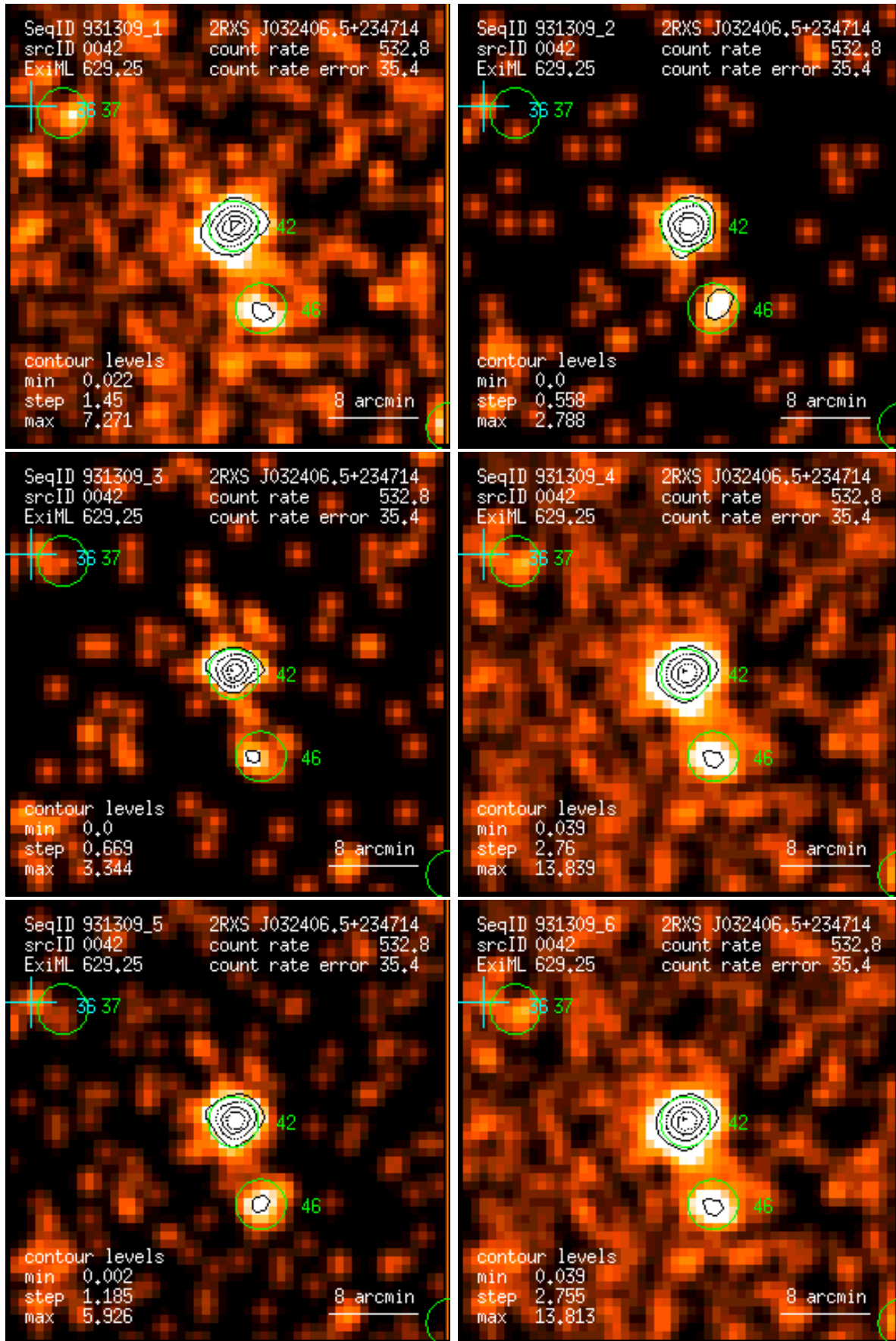
Figure 42: RASS 931309: detection 0042: band rate images, Gaussian filter: (1) PSPC channels 11 – 41, (2) 52 – 90, (3) 91 – 201, (4) 11 – 235, (5) 52 – 201, (6) 11 – 201. Broad band rates in counts/ks. Band rate contour levels in counts/ks/arcmin 2 .
